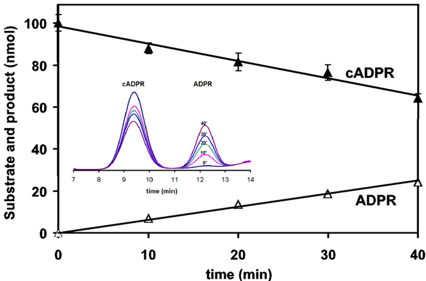
FIGURE 3. ADPRC catalyzes the hydrolysis of cADPR in a progressive way. ADPRC (5 \mu\text{g/ml} ) was incubated with 1 mM cADPR in 25 mM Tris-HCl, pH 8, for 10–40 min. The ADPR product was analyzed by HPLC.
