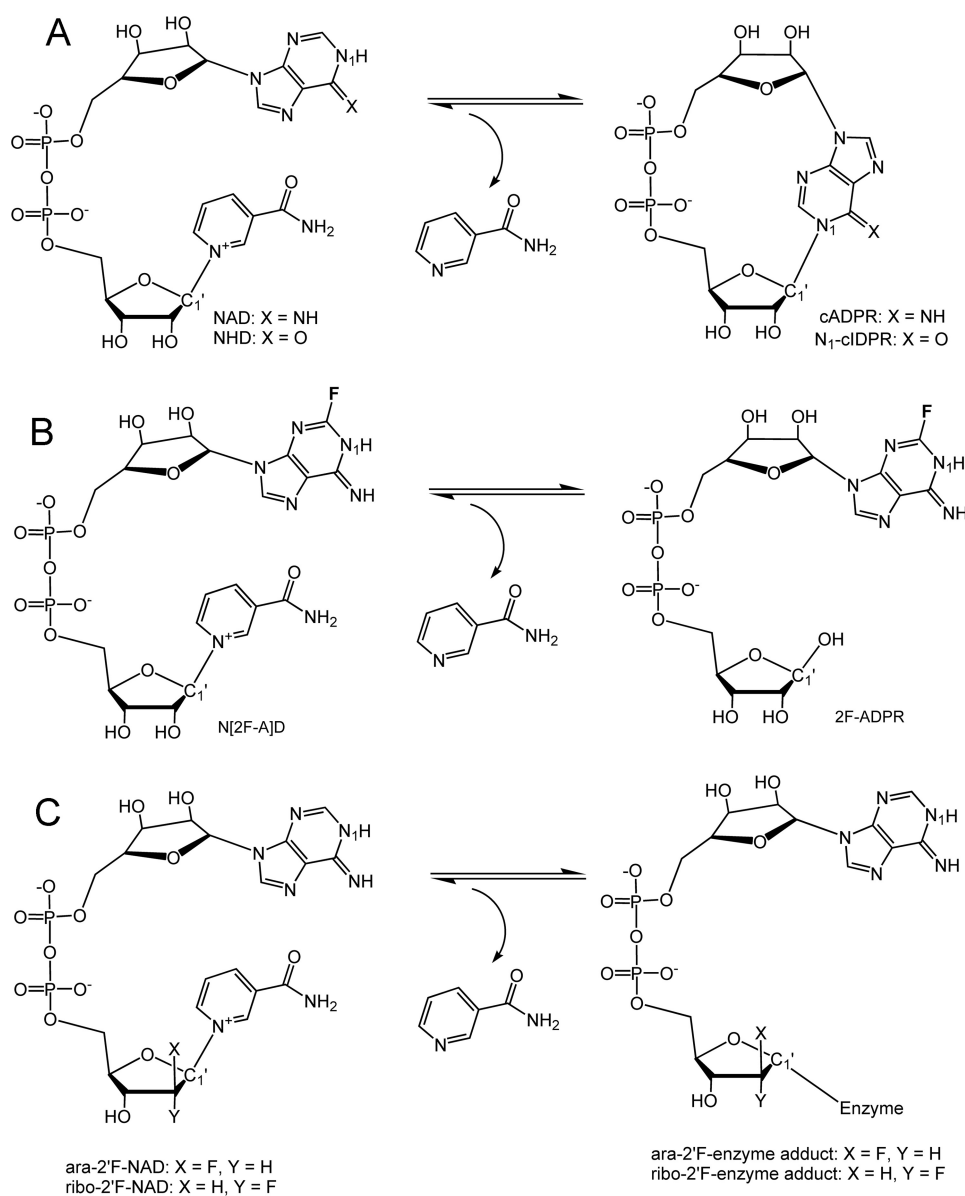
FIGURE 1. Schemes of cADPR formation and mechanistic analogs for substrate and product. A , the cyclization reaction producing cADPR from NAD is catalyzed by both ADPRC and CD38. The structural difference between cADPR and N1-cIDPR lies at the 6-position of purine ring (6-NH for cADPR; 6-O for N1-cIDPR). B , an analog of the substrate NAD, N(2F-A)D, is enzymatically converted to 2F-ADPR by ADPRC instead of cyclized to c(2F-A)DPR. The formation of cADPR from NAD requires the intramolecular attack of the reaction intermediate by the adenine N1 atom. The addition of a fluorine atom on the adjacent C2 atom of adenine prevents the cyclization from occurring. C , ara-2'F-NAD and ribo-2'F-NAD are analogs of NAD that inhibit the cyclization reaction by producing covalent adducts during the catalysis by CD38. Both analogs differ only in the orientation of their fluorine atoms at the 2'-position of the adenine ribose.
