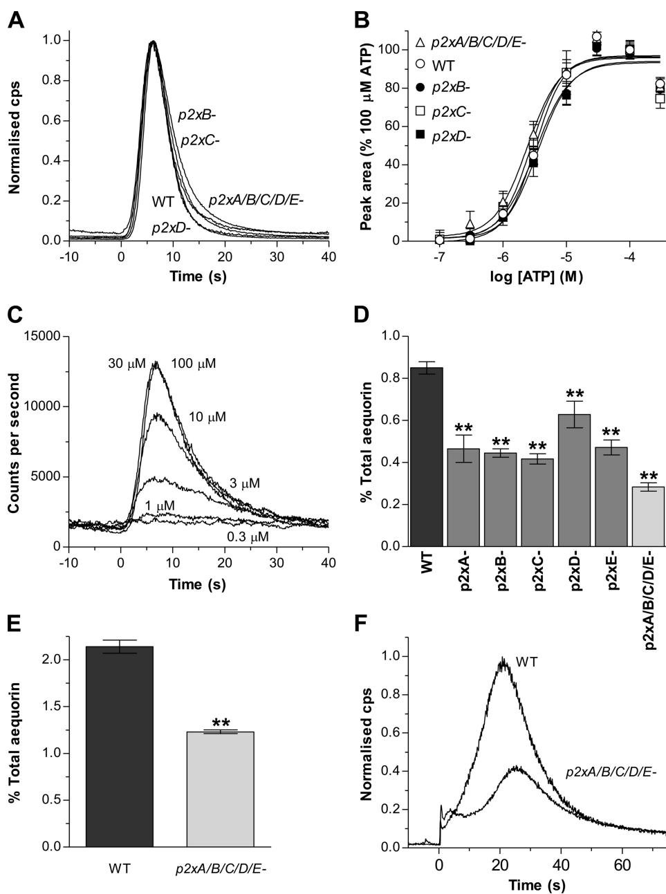
FIGURE 5. The response to extracellular purine nucleotides persist in p2x null strains. A , representative aequorin responses to ATP (30 \mu\text{M} ) in p2xB , p2xC , and p2xD single and p2xA/B/C/D/E quintuple null strains compared with wild type ( WT ). Cells were incubated with the cofactor benzyl-coelenterazine in HL-5 media ( 1 \times 10^7 cells/ml) to reconstitute functional aequorin and then transferred to MES development buffer (10 mM MES, 10 mM KCl, 0.25 mM \text{CaCl}_2 pH 6.8) ( 5 \times 10^6 cells/ml), and responses to ATP were monitored using a luminometer. The kinetics of the response to ATP is unaffected by p2x gene deletion. Traces are normalized to the maximal response for each individual strain to provide a direct comparison of time course. Time 0 corresponds to the application of agonist. B , ATP concentration response curves for WT and p2x null strains. Data are normalized to 100 \mu\text{M} ATP for each strain (mean \pm S.E., n \geq 5 for each data point from at least two independent experiments). C , representative concentration-dependent ATP responses in p2xA/B/C/D/E quintuple null cells. D , response magnitudes to ATP (30 \mu\text{M} ) expressed as percent total aequorin consumption for wild-type ( WT ) and p2x null strains. Data are presented as means \pm S.E. from 18 independent experiments for wild-type and six independent experiments with two independent clones for p2x null strains ( n \geq 30 ). E , the magnitude of the response to calmidazolium (2.5 \mu\text{M} ) is reduced in p2xA/B/C/D/E quintuple null cells compared with wild type ( WT ). Data are presented as mean percent total aequorin consumption from four independent experiments with two independent clones assayed for p2xA/B/C/D/E null cells ( n \geq 20 ). F , representative aequorin responses to calmidazolium (2.5 \mu\text{M} ) in wild-type and p2xA/B/C/D/E null cells. **, significant difference ( p < 0.01 ) compared with wild type.
