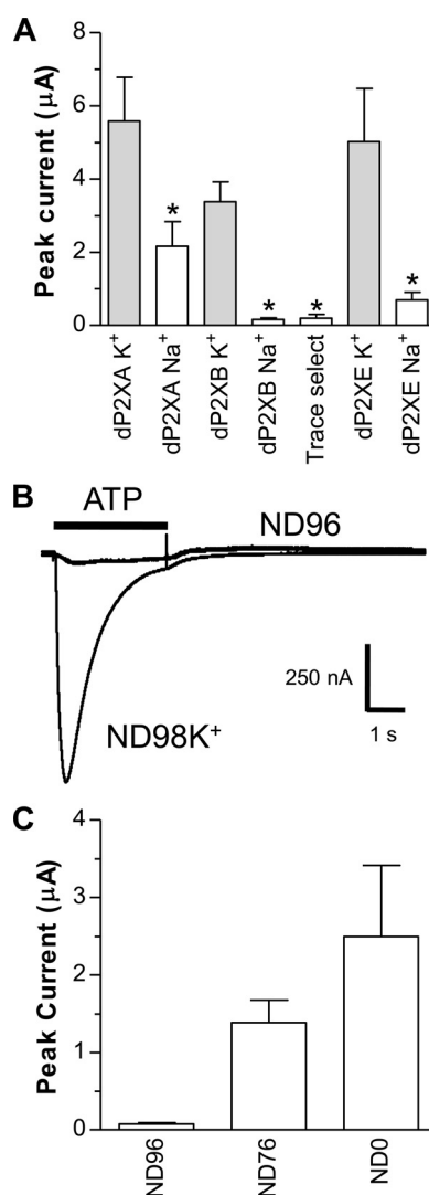
FIGURE 1. dP2X receptors are inhibited by Na + . Two-electrode voltage clamp recordings at a holding membrane potential of -70 mV were made from Xenopus oocytes expressing dP2X receptors. A , comparison of peak current amplitudes recorded in response to 3 mM ATP in extracellular recording solutions consisting either of ND96 (Na + based) or ND98K + (K + based) with both solutions at pH 6.2. Note inhibition of currents by Na + particularly for dP2XB and dP2XE channels. "Trace select" denotes ND96 extracellular recording solution made with ultrapure NaCl (Fluka 38979) for dP2XB. *, significant difference, p < 0.05 , compared with respective ND98K + current ( n = 7 ). B , direct comparison of current amplitudes in ND96 and ND98K + extracellular recording solutions (both pH 6.2) in the same dP2XB-expressing oocyte. Application of ATP (3 mM indicated by the bar) in ND96 was followed 5 min later by ATP application in ND98K + . C , mean current amplitudes in dP2XB-expressing oocytes after substitution of Na + in ND96 with NH 4 + . ND76 denotes ND96 with 20 mM NH 4 Cl substituting for 20 mM NaCl. ND0 denotes solution with zero Na + and 96 mM NH 4 Cl ( n = 7 ).
