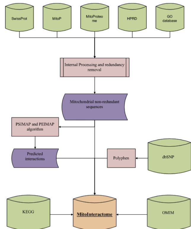
Figure 1 Flow chart for the construction of MitoInteractome. A schematic representation of the MitoInteractome database construction.
