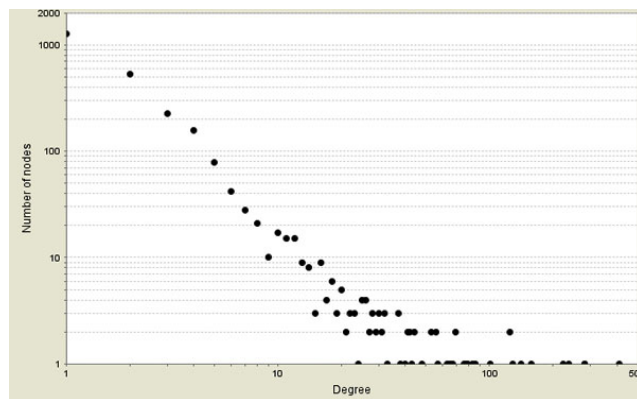
Figure 6 Plot of node degree distribution. The figure illustrates the node degree distribution for the aging network constructed.
