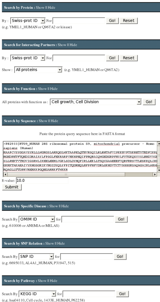
Figure 3 The graphical user interface for MitoInteractome. The graphical user interface for MitoInteractome providing facility to search by 1) Protein 2) Interacting partners 3) Function 4) Sequence 5) Disease association 6) SNP relation 7) Pathway association.
