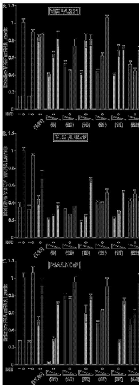
Figure 5. Gene-regulation effects measured by quantitative real-time RT-PCR for the oxime-linked polyamides 9-11 , 20-23 , 31-33 and 42-44 , and the hydroxylamine tail control compounds 5 , 16 , 27 , and 38 . Induced and uninduced control conditions are indicated by black bars, match core compounds by light grey bars, and mismatch core compounds by dark grey bars. Uninduced and induced control compounds without DMSO are on the left, and with 0.1% DMSO on the right. Errors shown are the fractional standard deviation. A) Effect on DFO-induced expression of VEGF by HRE-targeted match and mismatch polyamide cores in U251 cells at 1, 0.2, and 0.02 \mu\text{M} ; B) Effect on DFO-induced expression of VEGF by HRE-targeted match and mismatch polyamide cores in LNCaP cells at 10, 2 and 1 \mu\text{M} ; C) Effect
