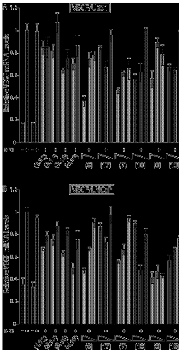
Figure 3. Quantitative real-time RT-PCR data showing the effect of HRE-targeted match compounds 1-4 , 6-8 and their mismatch congeners 12-15 , 17-19 on DFO-induced VEGF expression in cultured cells. Induced and uninduced control conditions are indicated by black bars, match core compounds by light grey bars, and mismatch core compounds by dark grey bars. Uninduced and induced control compounds without DMSO are on the left, and with 0.1% DMSO on the right. Errors shown are the fractional standard deviation. A) Expression of VEGF in cultured U251 cells under DFO-induced hypoxic conditions of match core control compounds 1-4 and mismatch core control compounds 12-15 at 1 \mu M concentration. Cells were treated with match compounds 6-8 and respective mismatch compounds 17-19 as 1, 0.2 and 0.02 \mu M cell culture media solutions. B) Expression of VEGF in cultured LNCaP cells under DFO-induced hypoxic conditions of match core control compounds 1-4 and mismatch core control compounds
