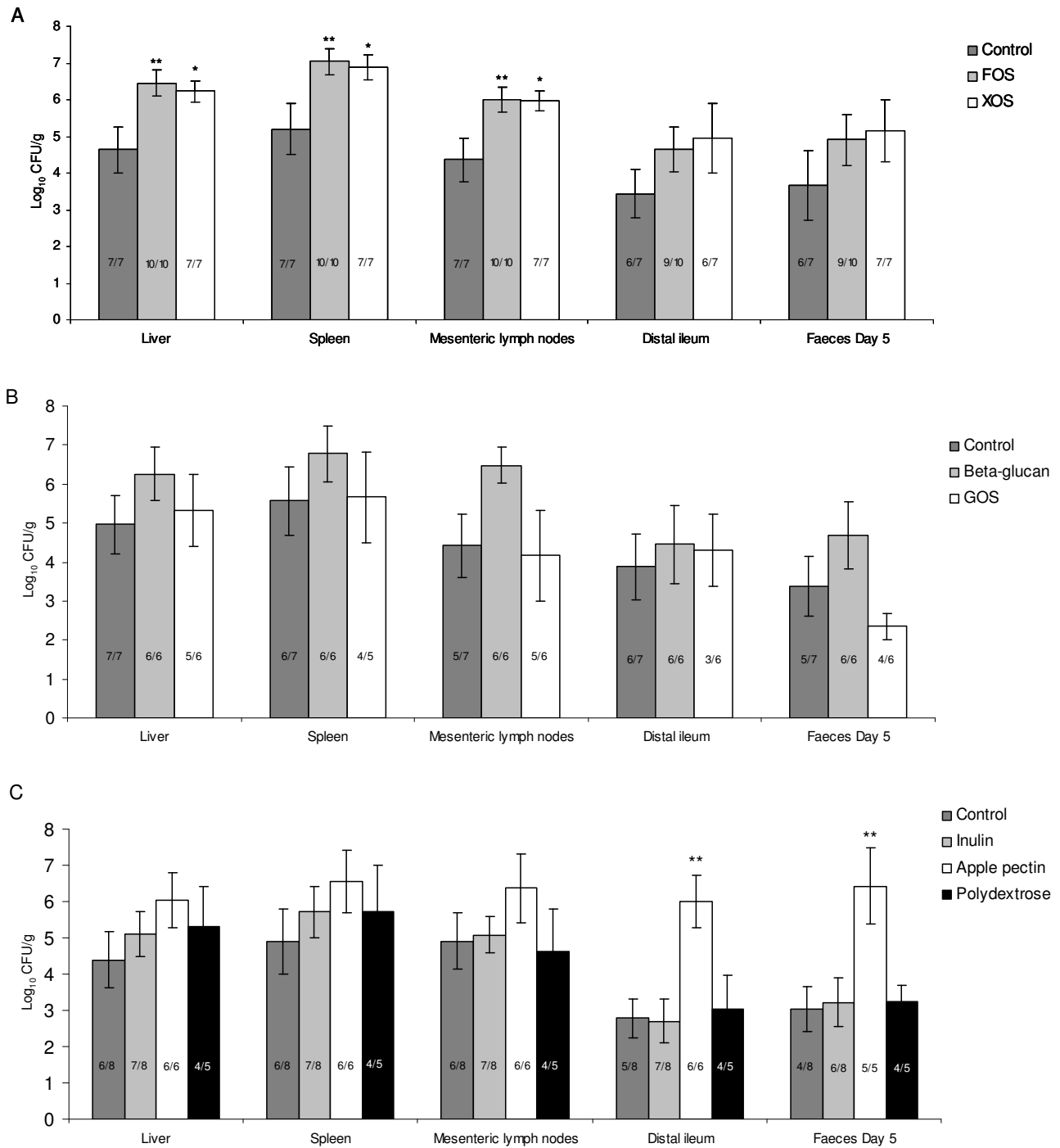
Figure 1 Salmonella counts in organs, distal ileum, and faeces. Enumeration of S. Typhimurium SL1344 from the liver, spleen, mesenteric lymph nodes, distal part of ileum and faeces from mice five days post challenge. A: Control, FOS and XOS; B: Control, beta-glucan and GOS; C: Control, inulin, apple pectin and polydextrose. Values represent means ± SEM. Prevalences of mice with detectable numbers of Salmonella in the organs are shown on the columns. *P < 0.05; **P < 0.01
