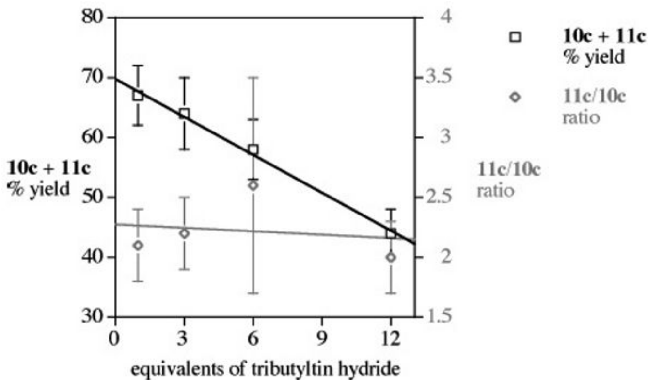
Figure 1. Yield and ratio of aromatic trapping products 10c/11c upon increasing [\text{Bu}_3\text{SnH}] .
