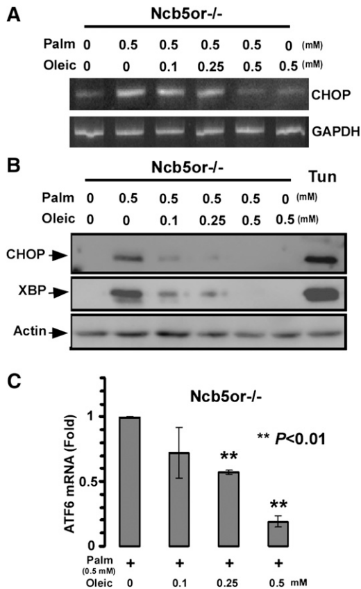
Fig. 5. Effect of oleic acid on palmitic acid induced ER stress. A, B: Hepatocytes were incubated with either 0 or 0.5 mM palmitate alone or 0.5 mM palmitate (Palm) mixed with increasing concentrations of oleic acid (0.1, 0.25 and 0.5 mM) for 12 h. A: Chop and GAPDH mRNA expression was determined by RT-PCR. B: Western blot determination of expression of CHOP and XBP-1 protein. C: After treatment of isolated hepatocytes with palmitate (0.5 mM) for 24 h, oleic acid was added at the indicated concentrations. After a further 12 h incubation, cells were collected for analysis of ATF6 mRNA. (n = 3 animals/genotype) Asterisks represent significant differences between presence and absence of oleate. Error bars indicate mean \pm SD.
