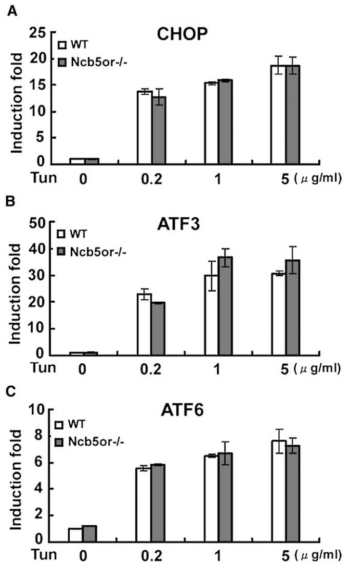
Fig. 6. Sensitivity to tunicamycin. Isolated primary hepatocytes from wild-type mice and NCB5OR null mice were treated for 12 h with increasing concentrations of tunicamycin. After cell collection, total RNA was extracted from each sample. Chop , ATF3 , and ATF6 mRNA were determined by quantitative PCR. No significant differences were noted between KO and WT cells at each dose of tunicamycin (n = 3 animals/genotype). Error bars indicate mean \pm SD.
