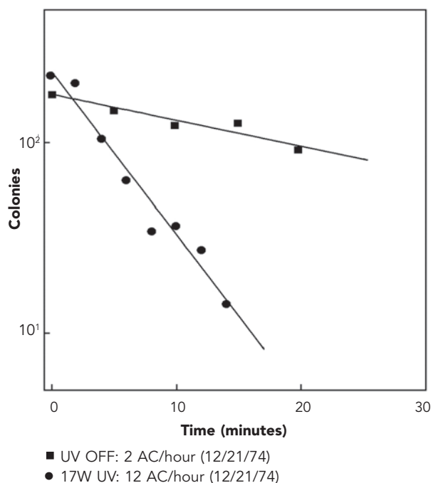
Figure 3. Disappearance rate of Bacillus Calmette-Guérin in a model room without upper-room UVGI and with a 17-watt upper-room UVGI lamp a,b
