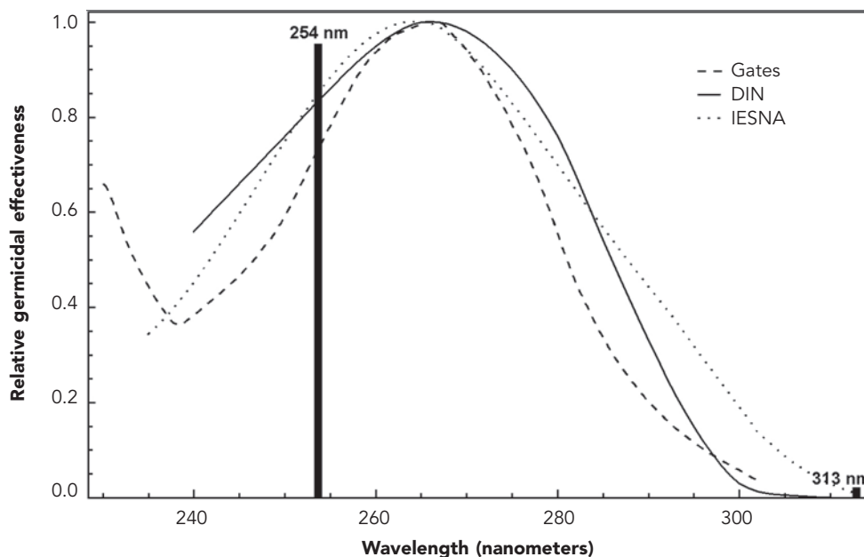
Figure 2. Gates’ original bactericidal action spectrum for Bacterium coli , a modern germicidal action spectra, b and the relative output of a low-pressure Hg germicidal lamp c,d
