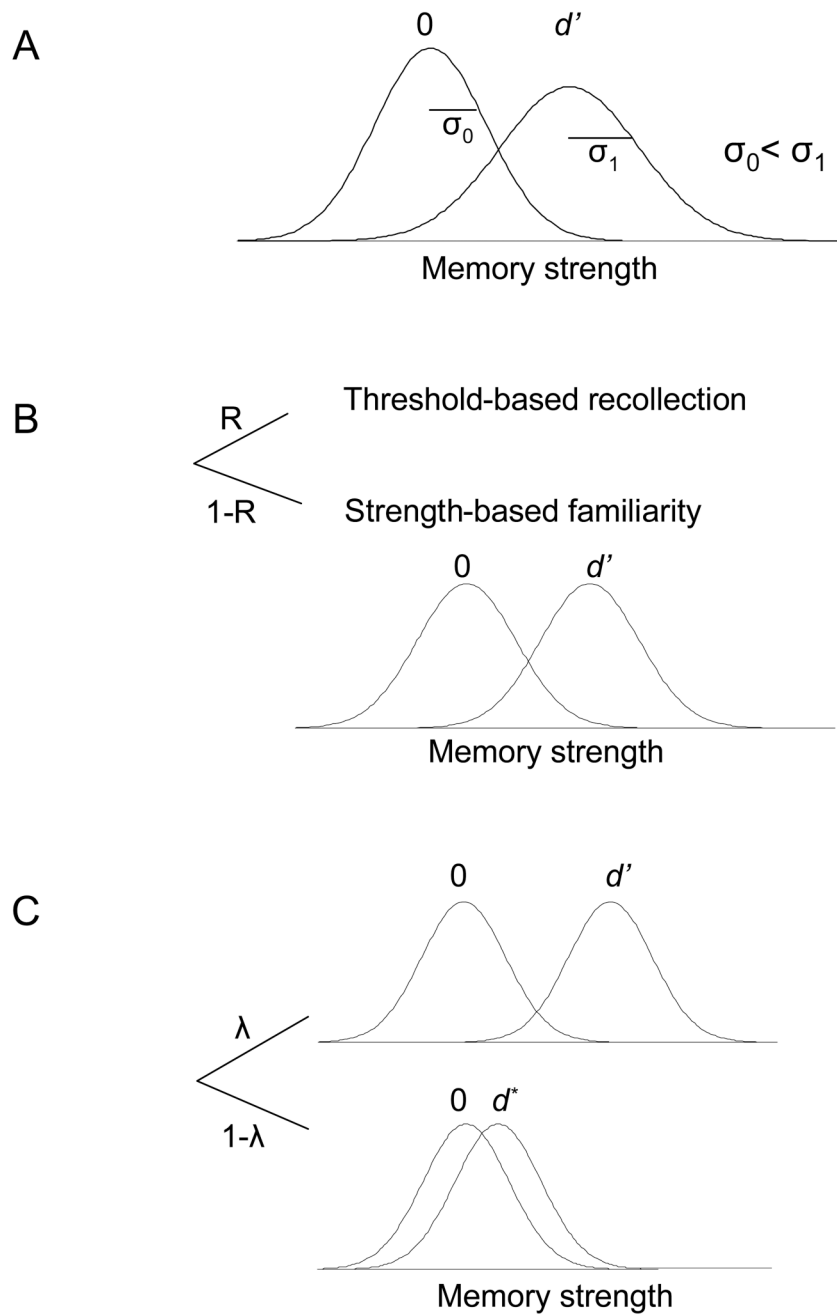
Figure 1. Three signal-detection models. (A) Unequal-variance signal-detection (UVSD) model; (B) Dual-process signal-detection (DPSD) model; (C) Mixture signal-detection (MSD) model.
