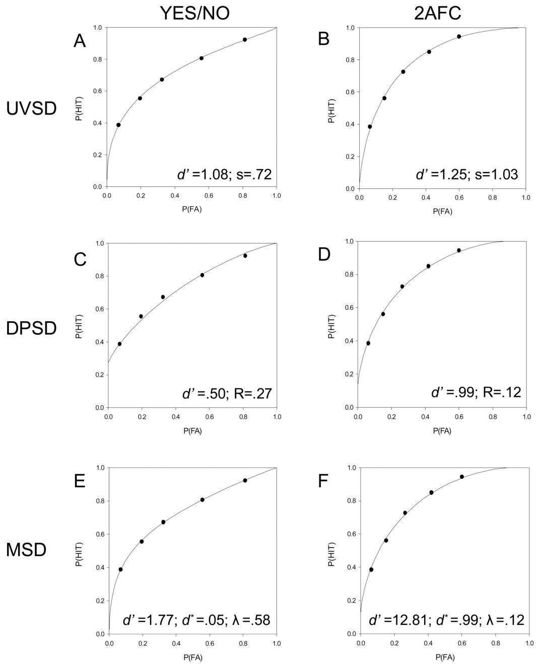
Figure 3. ROC curves for yes/no (left) and 2AFC (right) fits of the UVSD model (top: graphs A and B), DPSD model (middle: graphs C and D), and MSD model (bottom: graphs E and F).
