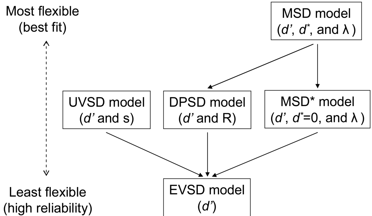
Figure 2. Nested hierarchy for the signal-detection models. Unidirectional, solid line arrows between models indicate subset relations between models. The bidirectional, dotted line arrow on the left-hand side represents the degree of the flexibility and reliability.
