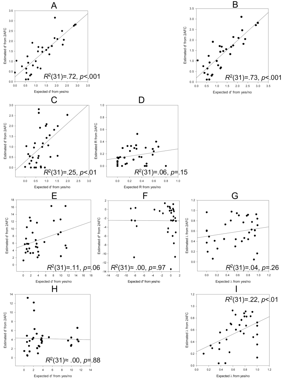
Figure 4. Scatter plots from the regression analysis. A = d'_{2AFC} expected from d'_{Yes/No} in the UVSD model; B = d'_{2AFC} expected from d'_{Yes/No} in the EVSD model; C = d'_{2AFC} expected from d'_{Yes/No} in the DPSD model; D = R_{2AFC} expected from R_{Yes/No} in the DPSD model; E = d'_{2AFC} expected from d'_{Yes/No} in the MSD model; F = d^*_{2AFC} expected from d^*_{Yes/No} in the MSD model; G = \lambda_{2AFC} expected from \lambda_{Yes/No} in the MSD model; H = d'_{2AFC} expected from d'_{Yes/No} in the MSD* model; I = \lambda_{2AFC} expected from \lambda_{Yes/No} in the MSD* model.
