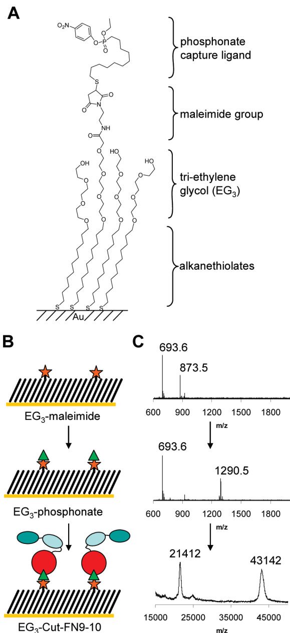
Figure 2. (A) SAMs presenting a phosphonate capture ligand for the covalent immobilization of cutinase–fibronectin fusion proteins. (B) Substrates were prepared by first treating a maleimide-terminated monolayer with a phosphonate ligand and then with a cutinase fusion protein to immobilize the FN fragments. (C) SAMDI mass spectrometry was used to confirm the masses of the ligands presented on the surface after each step.
