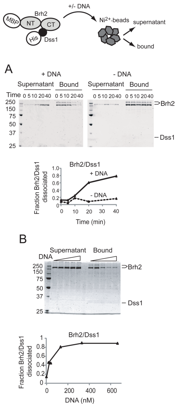
FIGURE 3. Dissociation of Brh2/Dss1 complexes. MBP-tagged Brh2 (represented as N-terminal and C-terminal lobes) complexes with His-tagged Dss1 (black ball) is mixed with Ni 2+ -NTA beads. A. Brh2/His-Dss1 complex (550 nM) was incubated at 37° in the presence or absence of DNA (130 nM unlabeled ss60mer). At the indicated times (min) Ni 2+ -NTA beads were added to pull down His-Dss1 either free or complexed with Brh2. Protein composition in the supernatant or bound fractions was determined by SDS gel electrophoresis. Protein was visualized by staining with SimplyBlue Safestain (Invitrogen). The time course of dissociation is shown graphically. B. Reactions mixes contained Brh2/His-Dss1 complex (550 nM) and increasing concentrations
