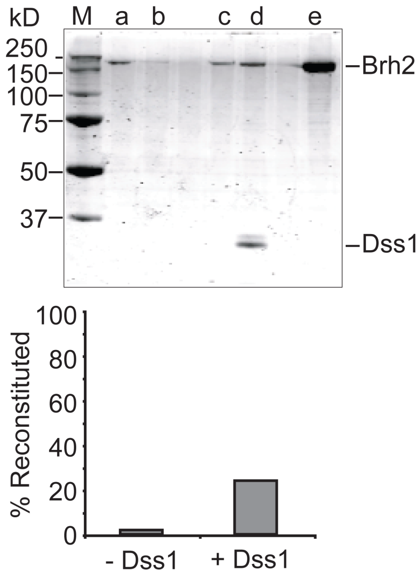
FIGURE 8. Reconstitution of the Brh2/Dss1 complex. Reaction mixtures containing Brh2 apoprotein were mixed with His-Dss1. After 1 hr at 4°, Ni 2+ -NTA beads were added, washed, then eluted with SDS sample buffer (80 µL). Aliquots (10 µL) of the supernatant (first wash) and bound fractions were separated by SDS gel electrophoresis. After staining with SimplyBlue Safestain, bands were quantitated using the Odyssey detection platform. Lane a -- supernatant, no Dss1; lane b -- bound, no Dss1; lane c -- supernatant, plus Dss1; lane d -- bound, plus Dss1; lane e -- 12.5% of total Brh2 apoprotein initially added to the reaction. M--size standards.
