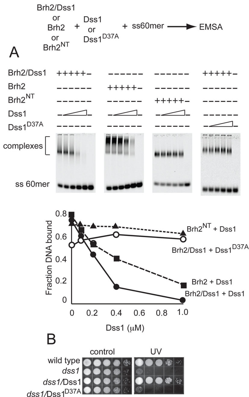
FIGURE 5. Dss1 attenuates DNA-binding activity of Brh2/Dss1 complex. A. To DNA binding reaction mixtures containing IRD800 labeled ss60mer (3.3 nM) and Brh2/His-Dss1, Brh2, or Brh2 NT (100 nM) was added increasing levels of His-Dss1 or His-Dss1 D37A to the lanes as indicated (0.1, 0.2, 0.4, and 1.0 μM, respectively). After incubation for 20 min, DNA binding was determined. B. Survival of dss1 deletion strain expressing Dss1 or Dss1 D37A was determined after a UV dose of 120 J/m 2 .
