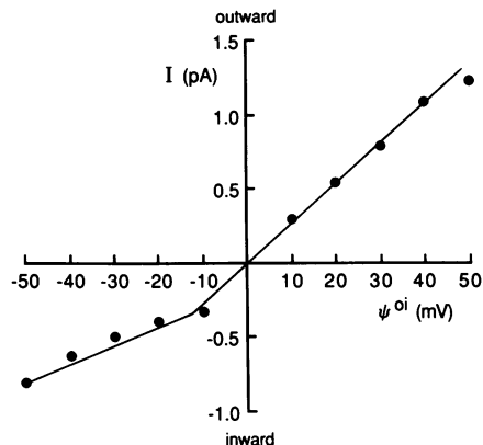
FIG. 3. Current–voltage relation of an excised patch containing a channel that was activated after the addition of glycine to the bathing solution. The patch of membrane was bathed symmetrically with 150 mM KCl and 106 nM \text{Ca}^{2+} (Ca EGTA buffer, pH 7.2). \psi^{oi} is the electrical potential difference across the patch with reference to the outer solution. An outward current is defined as a cationic current leaving the cell (entering the pipette).
