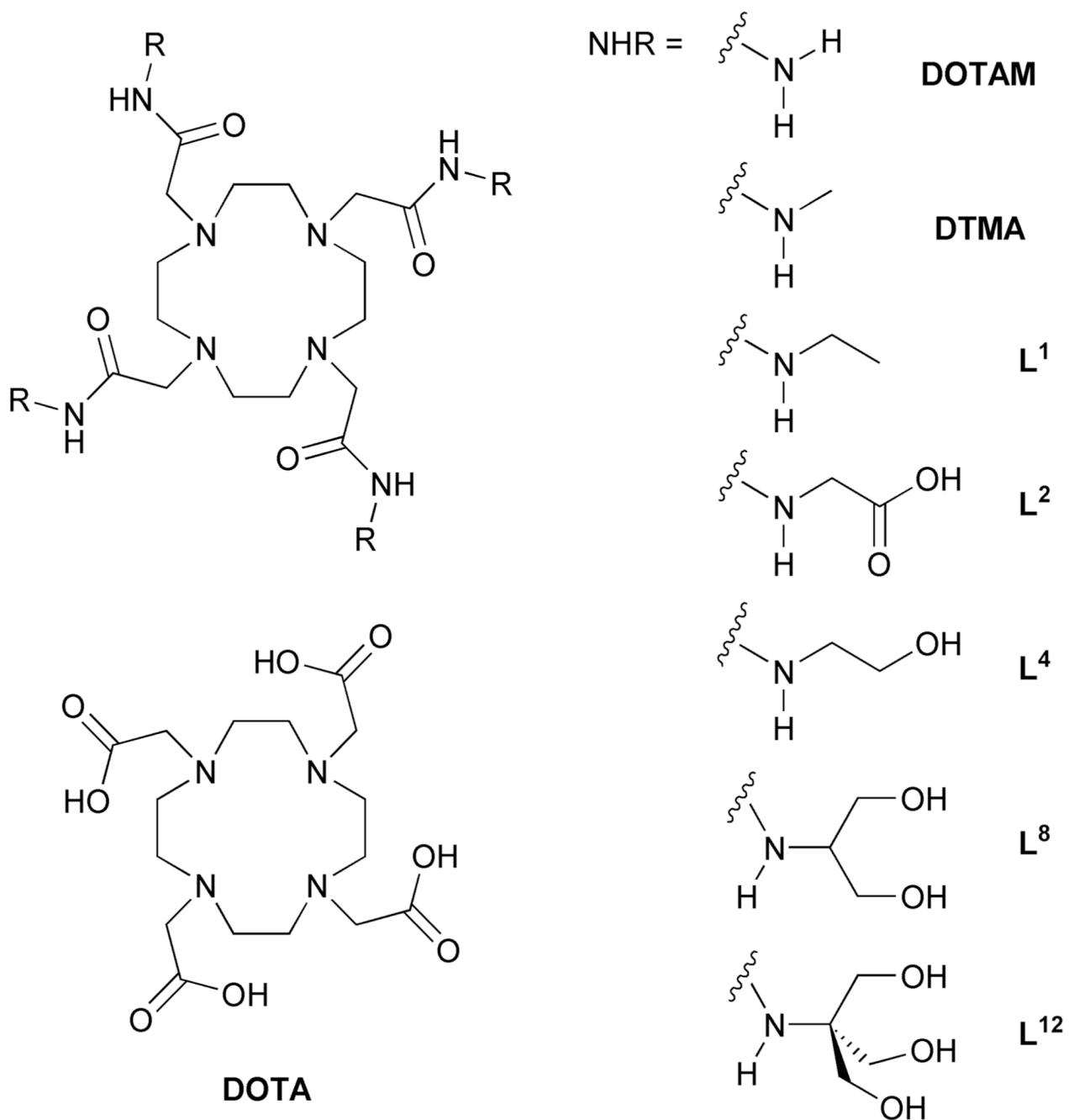
Chart 2. The structures of DOTA-tetraamide ligands, potential PARACEST agents
