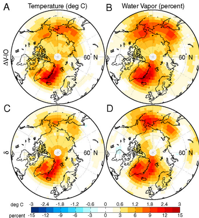
Fig. 2. (A) The anomaly ( \Delta V - IO ) in near-surface atmospheric temperature in degrees Celcius (deg C) between a model experiment where trees are introduced on bare ground north of 60^\circ\text{N} and a corresponding control run with no added trees. (B) The same as (A) for column water vapor in percent. (C) The difference \delta(\Delta V - IO - \Delta V - FO) in near-surface atmospheric temperature in deg C between two anomalies where trees are introduced on bare ground north of 60^\circ\text{N} , one with an interactive ocean model (V-IO), and the other with fixed ocean and sea-ice (V-FO). (D) The same as (C) for column water vapor in percent.
