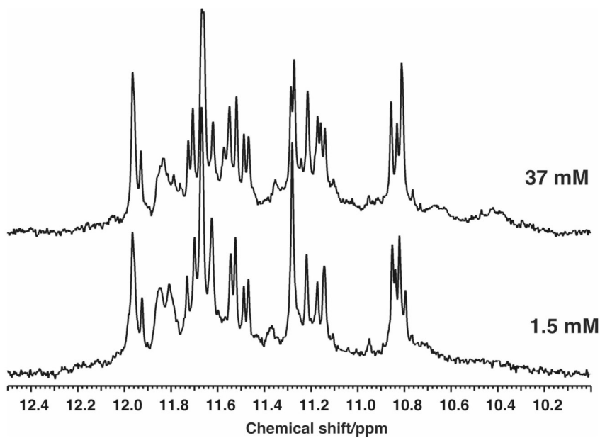
FIGURE 5. 1 H NMR spectra of Tel22 as a function of KCl concentration showing the imino proton region of the NMR spectra of Tel22 (178 μM) at 1.5 mM and 37 mM KCl at 10 °C (A) and 25 °C (B).
