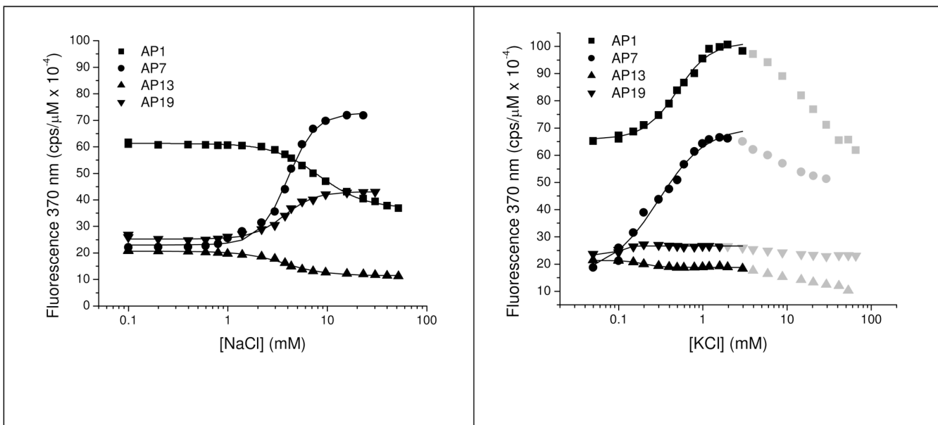
FIGURE 3. Titration curves for cation-induced folding of 2-AP derivatives of Tel22 assessed by changes in fluorescence emission at 370 nm. Panel A shows the dependence of the fluorescence intensity on [NaCl] and panel B shows the dependence of the fluorescence intensity on [KCl] for the derivatives of Tel22 substituted with 2-AP at the indicated positions. The points represent the experimental fluorescence intensities (normalized to 1 μM oligonucleotide concentration) and the line shows the fit of the data points to eq. 3 determined by non-linear least squares as described in the text. The data points were corrected for day-to-day variations in excitation intensity. The data points shown in grey in Panel B were not included in the fitting. The optimized fitting parameters are given in Table 1. Conditions: [Tel22] = 0.7 – 1.0 μM in 10 mM Bu 4 AmP, 1 mM EDTA, pH 7.0, 25 °C, excitation wavelength = 305 nm.
