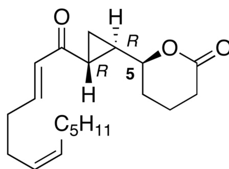
Eicosanoid
