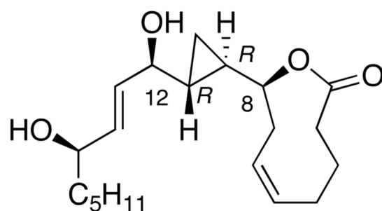
Halicholactone
