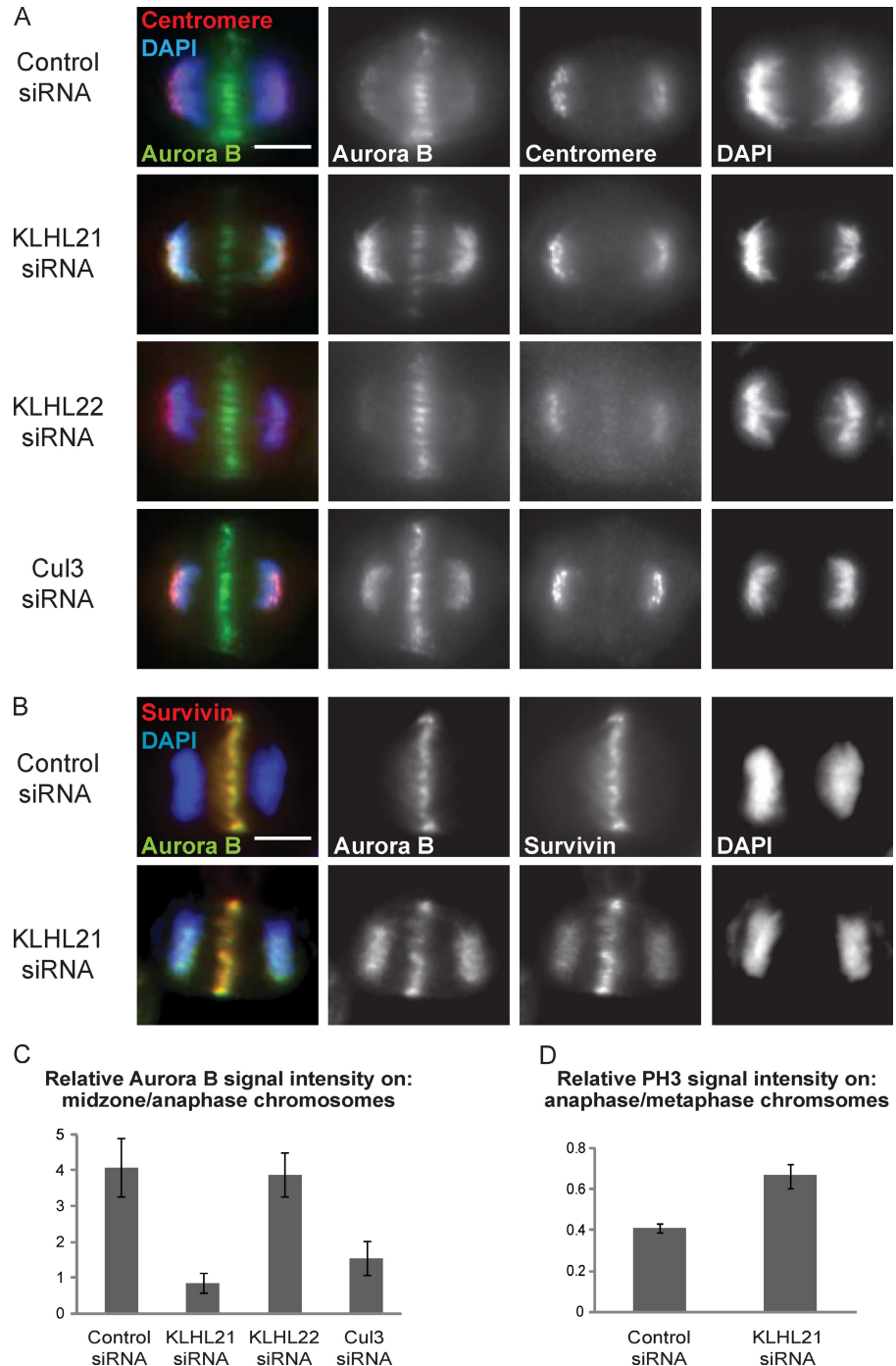
Figure 2. KLHL21 is a novel regulator of the CPC. (A and B) HeLa cells treated with the indicated siRNAs were analyzed by IF for Aurora B and centromeres (A) or survivin (B). DNA was stained with DAPI. (C) Quantification of the relative intensity of Aurora B from A. The intensity on the midzone was divided by the intensity on anaphase chromosomes ( n = 20 ). (D) HeLa cells treated with control or KLHL21 siRNA were analyzed by IF for Aurora B and Ser10-phosphorylated histone H3 (PH3). Quantification of the relative intensity of Ser10-phosphorylated histone H3 is shown. The intensity on anaphase chromosomes was divided by the intensity on metaphase chromosomes ( n = 20 ). (C and D) Bars represent the mean with standard deviation of three independent experiments. Bars, 5 \mu\text{m} .
