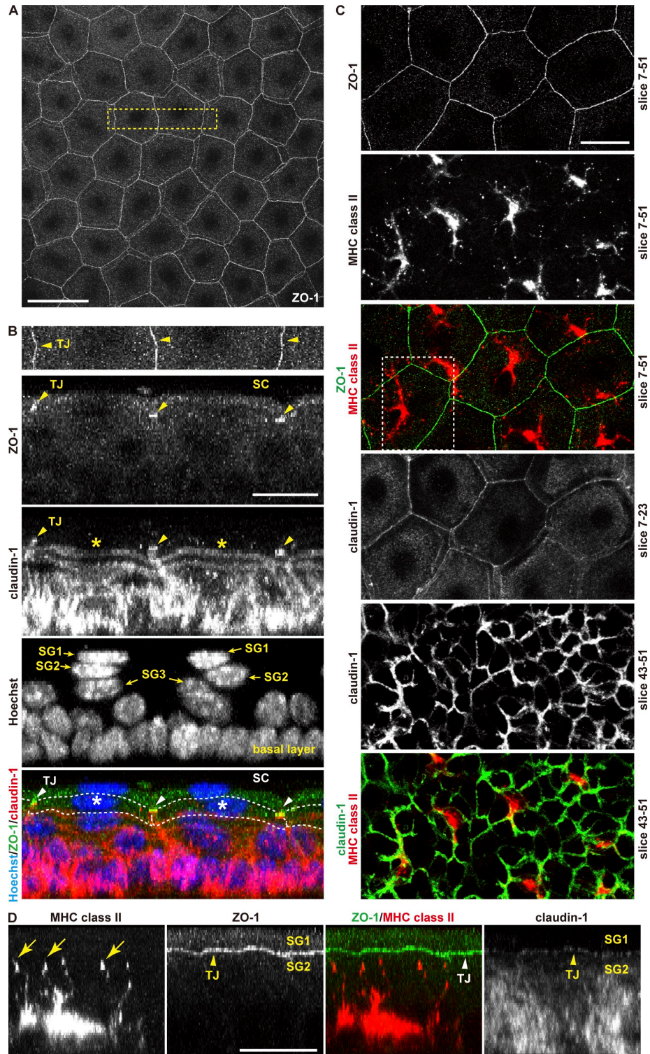
Figure 1. 3D visualization of epidermal TJs and LCs. (A) TJ network visualized by anti-ZO-1 antibody in epidermal sheet demonstrated en face by confocal microscopy. Bar, 50 \mu m. (B) A 90° rotation image of the boxed area in A. The top shows an en face image of ZO-1 staining followed by rotation images stained for the indicated TJ molecules. Among the three layers of granular layer, SG1 to SG3, TJs (arrowheads) were found exclusively in the SG2 layer (asterisk and dashed lines), and rotation images display TJs as bright dots with intense ZO-1 and claudin-1 signals (see Video 1). (C) TJs and LCs in unperturbed skin. Z-slice numbers are indicated in each panel. ZO-1 and claudin-1 colocalized at KC-KC TJs, and LCs (MHC II + ) coexpressed claudin-1 at high levels. (D) A 90° rotation image of the boxed area in C (see Video 2). Tips of LC dendrites (arrows) localized within TJ barriers (arrowheads). Bars, 20 \mu m. Data presented is representative of five mice.
