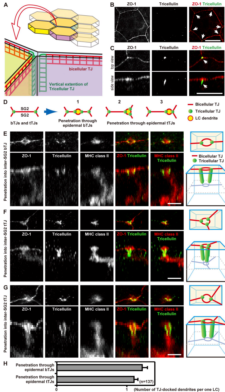
Figure 3. tJ formation at the TJ penetration point of LC dendrites. (A) Schematic structure of TJs at cell–cell contacts. TJ strands extend vertically below at tricellular contacts to form tTJs (Ikenouchi et al., 2005). (B and C) 3D reconstruction of epidermal sheet stained for ZO-1 and the tTJ protein tricellulin. Tricellulin appears as bright dots (B, arrows) when observed en face, but is found to extend vertically below in 90° rotated images (C, arrows). Bars, 20 \mu m. (D) Schematic representation of three patterns by which LC dendrites penetrate bTJs or tTJs at the SG2 layer. (E–G) 3D reconstruction images of LC dendrites penetrating TJs as modeled in D (see Video 3). Top rows of each show en face images and bottoms present 90° rotation images accompanied by schematic drawings on the right of each row. Bars, 5 \mu m. (H) Numbers of bTJ- and tTJ-docked dendrites per LC. The number of dendrites that docked with or penetrated TJs was counted on activated LCs after 12 h of tape stripping. Error bars represent SEM. Data presented in A–G is representative of three mice and data in H of three independent experiments.
