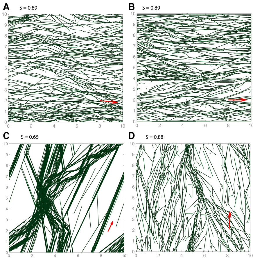
Figure 5. Simulation snapshots at t = 60 min using kinetic parameters from wild type at 31^\circ\text{C} . (A) Entrainment at shallow angles ( <40^\circ ) and no collision-induced catastrophe ( p_{cat} = 0 ). (B) A biased, transverse dominant angle that arises if two edges (here, the top and bottom) induce catastrophe. This provides a possible mechanism for selecting a direction transverse to the cell elongation axis. (C) Sparse array that results if all nucleation is branched MT-dependent nucleation. (D) Moderately sparse array arising from a combination of MT-dependent and MT-independent nucleation.
