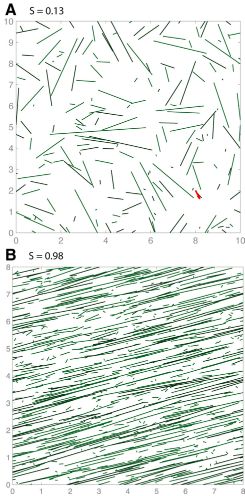
Figure 1. Simulation snapshots at t = 60 min with collision-induced catastrophe only, using parameters from wild type at 31°C (Kawamura and Wasteneys 2008) (A) and collision-induced pauses, using the single-state model of Baulin et al. (2007) (B).
