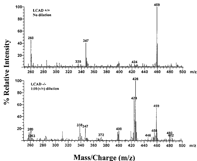
FIG. 4. Butyl-ester acylcarnitine profiles of bile specimens obtained using precursor-ion scanning (parent of m/z 85) electrospray/tandem mass spectrometry. Mice were sacrificed after overnight fast (18–20 hr), and bile specimens were collected as spots on filter paper. (Top) LCAD +/+ (normal control), no dilution. (Bottom) LCAD -/- (LCAD-deficient), 1:10 (vol/vol) dilution. Internal standards: m/z 263, d3-acetylcarnitine; m/z 347, d3-octanoylcarnitine; and m/z 459, d3-palmitoylcarnitine. Peak identification: m/z 260, acetylcarnitine (C 2 ); m/z 372, decanoylcarnitine (C 10 ); m/z 400, dodecanoylcarnitine (C 12 ); m/z 424, tetradecadienoylcarnitine (C 14:2 ); m/z 426, tetradecenoylcarnitine (C 14:1 ); m/z 456, palmitoylcarnitine (C 16 ); m/z 480, linoleylcarnitine (C 18:2 ); m/z 482, oleylcarnitine (C 18:1 ).
