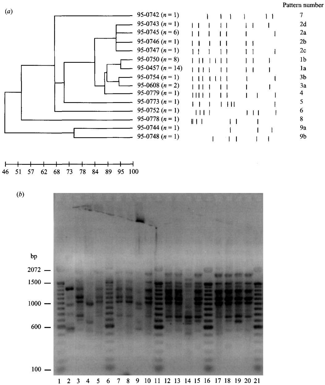
Fig. 4. REP-PCR of Vibrio isolates. The dendrogram shown (a) was constructed using digitized information from agarose gels as outlined in Materials and Methods. Strain numbers of representative isolates are given for each banding pattern, and numbers in parentheses indicate the number of isolates found for each pattern. The scale at bottom represents an arbitrary measure of pattern differences. A representative agarose gel is shown (b). The samples included were as follows, with isolates other than toxigenic V. cholerae designated and REP pattern numbers in parentheses: lane 1, size standard; lane 2, 95-0742 ( V. alginolyticus ; pattern 7); lane 3, 95-0743 (pattern 2d); lane 4, 95-0744 ( V. parahaemolyticus ; pattern 9a); lane 5, 95-0745 (pattern 2a); lane 6, size standard; lane 7, 95-0746 (pattern 2b); lane 8, 95-0747 (pattern 2c); lane 9, 95-0748 ( V. parahaemolyticus ; pattern 9b); lane 10, 95-0749 (pattern 2a); lane 11, size standard; lane 12, 95-0750 (pattern 1b); lane 13, 95-0751 (pattern 1b); lane 14, 95-0752 (non-toxigenic environmental V. cholerae ; pattern 6); lane 15, 95-0753 (pattern 1b); lane 16, size standard; lane 17, 95-0754 (pattern 3b); lane 18, 95-0755 (pattern 1b); lane 19, 95-0756 (pattern 1b); lane 20, 95-0757 (pattern 1a); lane 21, size standards. Sizes of the DNA size standard are indicated at the left of the gel.
