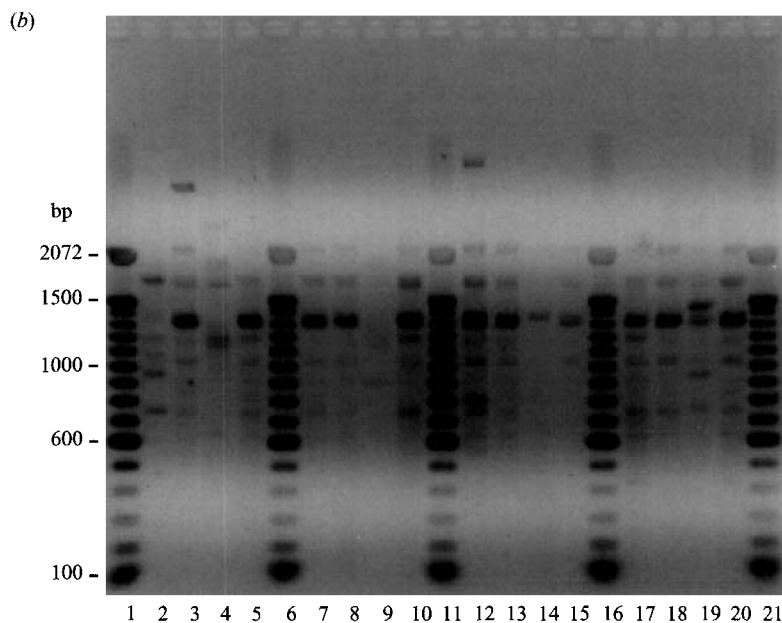
Fig. 3. ERIC-PCR of Vibrio isolates. The dendrogram (a) was constructed using digitized information from agarose gels as outlined in Materials and Methods. Strain numbers of representative isolates are given for each banding pattern, and numbers in parentheses indicate the number of isolates found for each pattern. The scale at bottom represents an arbitrary measure of pattern differences. A representative agarose gel is shown (b). The samples included were as follows, with isolates other than toxigenic V. cholerae designated and ERIC pattern numbers in parentheses: lane 1, size standard; lane 2, 95-0742 ( V. alginolyticus ; pattern 6); lane 3, 95-0743 (pattern 1d); lane 4, 95-0744 ( V. parahaemolyticus ; pattern 7a); lane 5, 95-0745 (pattern 2a); lane 6, size standard; lane 7, 95-0746 (pattern 1a); lane 8, 95-0747 (pattern 2a); lane 9, 95-0748 ( V. parahaemolyticus ; pattern 8); lane 10, 95-0749 (pattern 2a); lane 11, size standard; lane 12, 95-0750 (pattern 5a); lane 13, 95-0751 (pattern 1a); lane 14, 95-0752 (non-toxigenic environmental V. cholerae ; pattern 9); lane 15, 95-0753 (pattern 1a); lane 16, size standard; lane 17, 95-0754 (pattern 2a); lane 18, 95-0755 (pattern 1a); lane 19, 95-0756 (pattern 2d); lane 20, 95-0757 (pattern 2a); lane 21, size standards. Sizes of the DNA size standard are indicated at the left of the gel.
