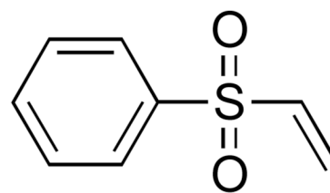
phenyl vinyl sulfone
