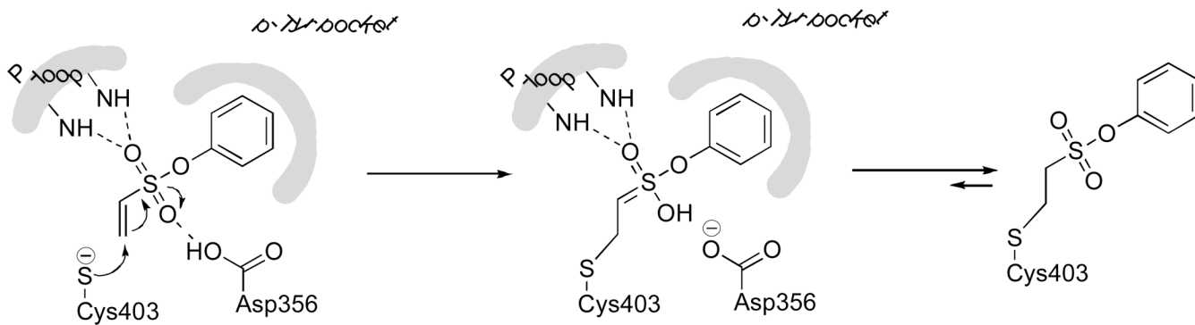
Figure 6. Mechanism of YopH inactivation by PVSN.
