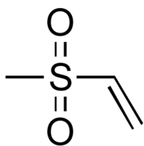
methyl vinyl sulfone
