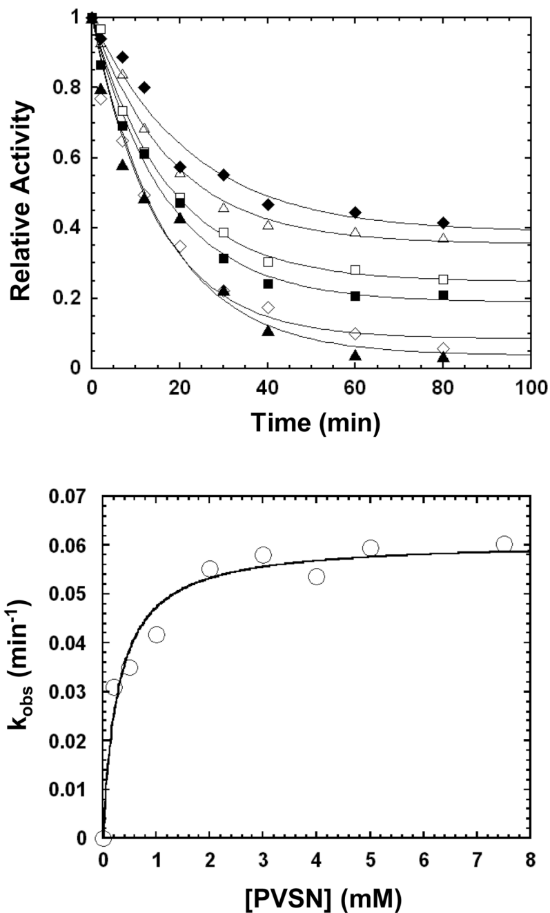
Figure 2. Kinetics of YopH inactivation by phenyl vinyl sulfonate. A. Time and concentration dependence of YopH inactivation by phenyl vinyl sulfonate. The experimental points are represented by various symbols and the line connecting them is the fitted line to equation 1 to yield pseudo-first order rate constant k_{obs} . Probe concentrations were as follows: \blacklozenge , 1 mM; \triangle , 2 mM; \square , 3 mM; \nabla , 5 mM; \blacktriangle , 7.5 mM; and \Gamma , 10 mM. B. Concentration dependence of the pseudo-first-order rate constants k_{obs} for phenyl vinyl sulfonate-mediated YopH inactivation. The points are experimental and the line connecting them is the fitted line to equation 2.
