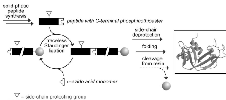
FIG. 4. Strategy for the chemical synthesis of proteins by iterative cycles of solid-phase peptide synthesis and solid-phase Staudinger ligation.
