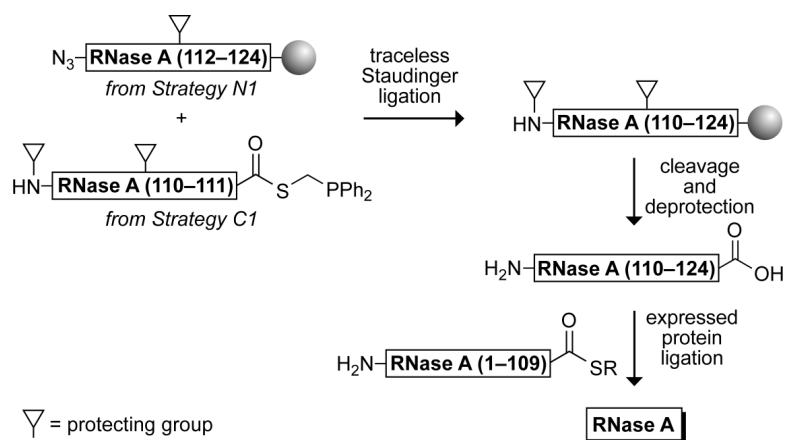
FIG. 3. Route for the assembly of RNase A with solid-phase peptide synthesis, Staudinger ligation, and expressed protein ligation.
