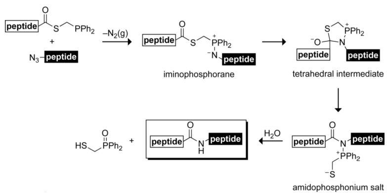
FIG. 1. Putative mechanism for the traceless Staudinger ligation of two peptides.
