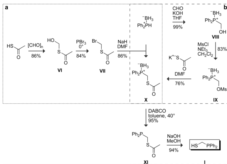
FIG. 2. Routes for the synthesis of (diphenylphosphino)methanethiol ( I ).
