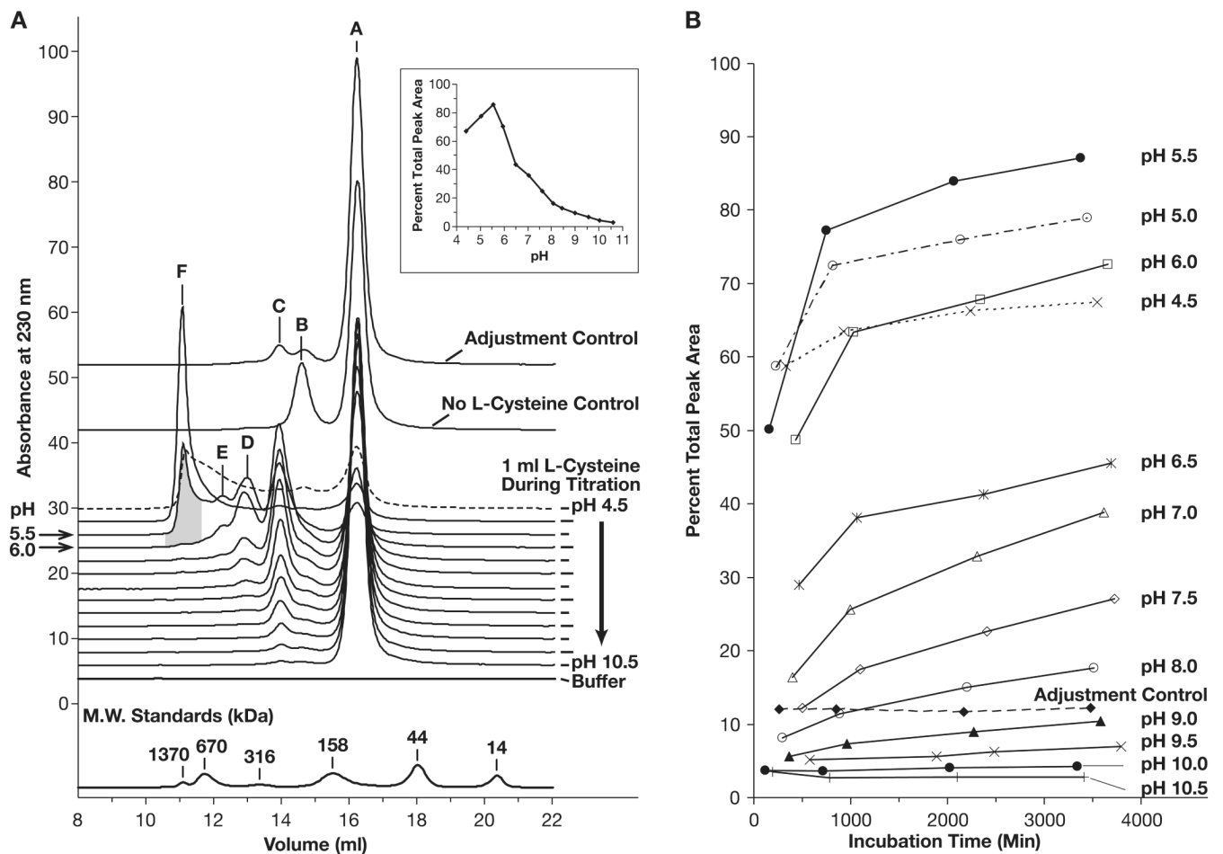
Fig. 6. Analysis of cysteine-stabilized F1-V MN non-covalent self-association (ADM). (Panel A) Stacked HPLC-SEC traces after incubation at 4 °C for 55–64 h at pH 4.5–10.5. The ‘Adjustment Control’ sample was derived from the pH 4.5-sample that was immediately back-titrated to pH 10.0. Peak solution state assignments were based on SEC-MALLS MW determinations (Fig. 8). Peak A, F1-V monomer; Peak B, F1-V (S-S) dimer (DTT-sensitive); Peak C, F1-V (NC) dimer (DTT-insensitive); Peak D, F1-V trimer; Peak E, F1-V multimer less than 0.5 MDa; Peak F, multimer, 0.5 to 6 MDa. The L-cysteine-free control at pH 9.9 established the F1-V (S-S) dimer position (Peak B). (Panel 1, Inset) Plot of the percentage of integrated peak area contained in dimer and multimer peaks as a function of incubation pH after 55–64 h. incubation (Panel B) Related plots of the percent integrated peak area contained in dimer and multimer peaks as a function of time and pH between 0 and 64 h incubation at 4 °C.
