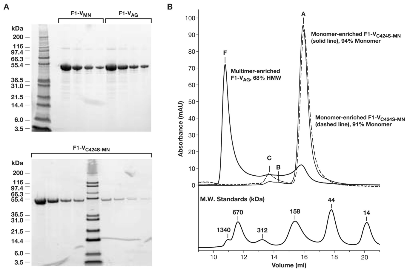
Fig. 5. (Panel A) SDS-PAGE analysis of final preparations. (Top) Comparison of F1-V MN before and after conversion to F1-V AG , loaded with two-fold dilution series starting at 9.2 µg/well; (Bottom) F1-V C424S-MN loaded starting at 9.6 µg/well. (Top, Lane 1, Bottom Lane 5) Mark 12 MW marker. (Panel B) Overlaid HPLC-SEC profiles of final F1-V MN (pH 9.9), F1-V C424S-MN (pH 9.9), and F1-V AG (pH 5.0) preparations. F1-V monomer eluted at an anomalous apparent molecular size of 100 kDa relative to high MW size standards (bottom).
