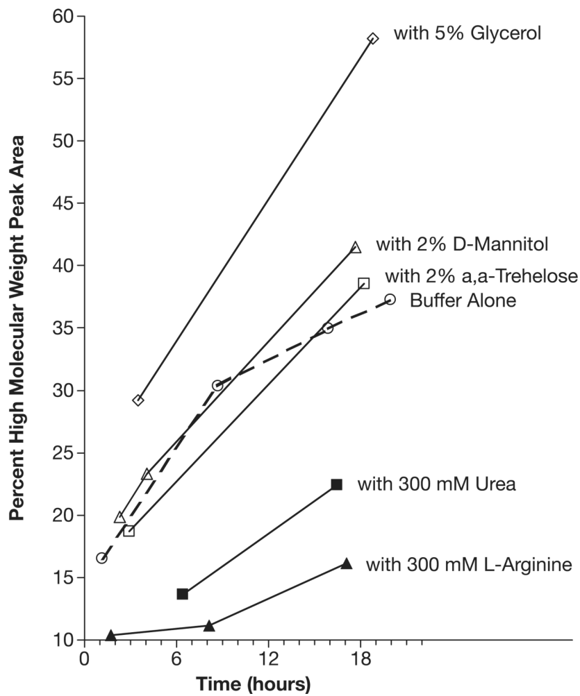
Fig. 7. Additive-induced F1-V non-covalent multimer-content modulation at pH 6.5 (ADM).
