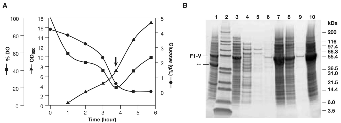
Fig. 3. (Panel A) Fermentation time course for cultivation of E. coli , BLR130 transformed with plasmid pW731 expressing F1-V. Arrow, induction with 1 mM IPTG, 0.2% arabinose (ADM). (Panel B) Sypro Ruby-stained, reduced SDS-PAGE analysis of F1-V MN recovery (ADM). Pellets were first prepared by ~25-fold dilution into 2x reducing running buffer. Loadings were 20 \mu L/well or 40 \mu L/well (lanes 4, 5, and 6). Lanes: 1) washed initial pellet lysate; 2) Mark 12 molecular mass markers (Invitrogen); 3) lysate supernatant; 4) pH 4.8 supernatant; 5) 1 st pH 4.8 rinse; 6) 2 nd pH 4.8 rinse; 7) pH 4.8 pellet; 8) post resolubilization and pellet; 9) 2 nd pH 4.8 step supernatant; 10) 2 nd pH 4.8 step pellet.
