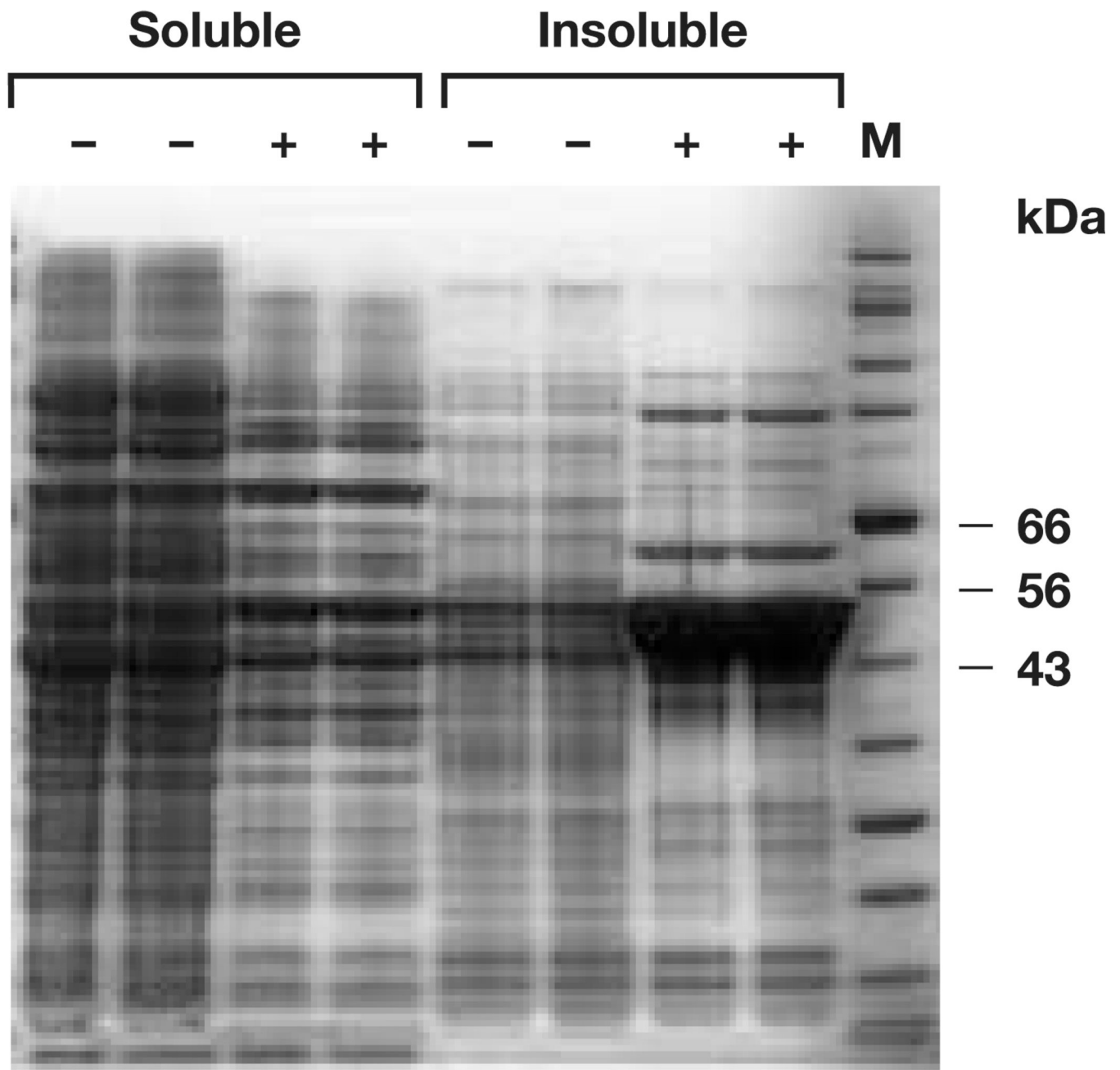
Fig. 2. Simply Blue-stained (Invitrogen), reduced SDS-PAGE analysis of F1-V C424S expression for whole broth soluble and insoluble fractions before (-) and after (+) IPTG induction. Lane M - protein molecular mass standard. The calculated molecular mass of F1-V C424S monomer is 53 kDa. Cells and supernatants were mixed with 4 x LDS sample buffer and heated at 70 °C for 10 min before electrophoresis through Invitrogen NuPAGE 4–12% Bis-Tris gels, using MOPS SDS running buffer.
