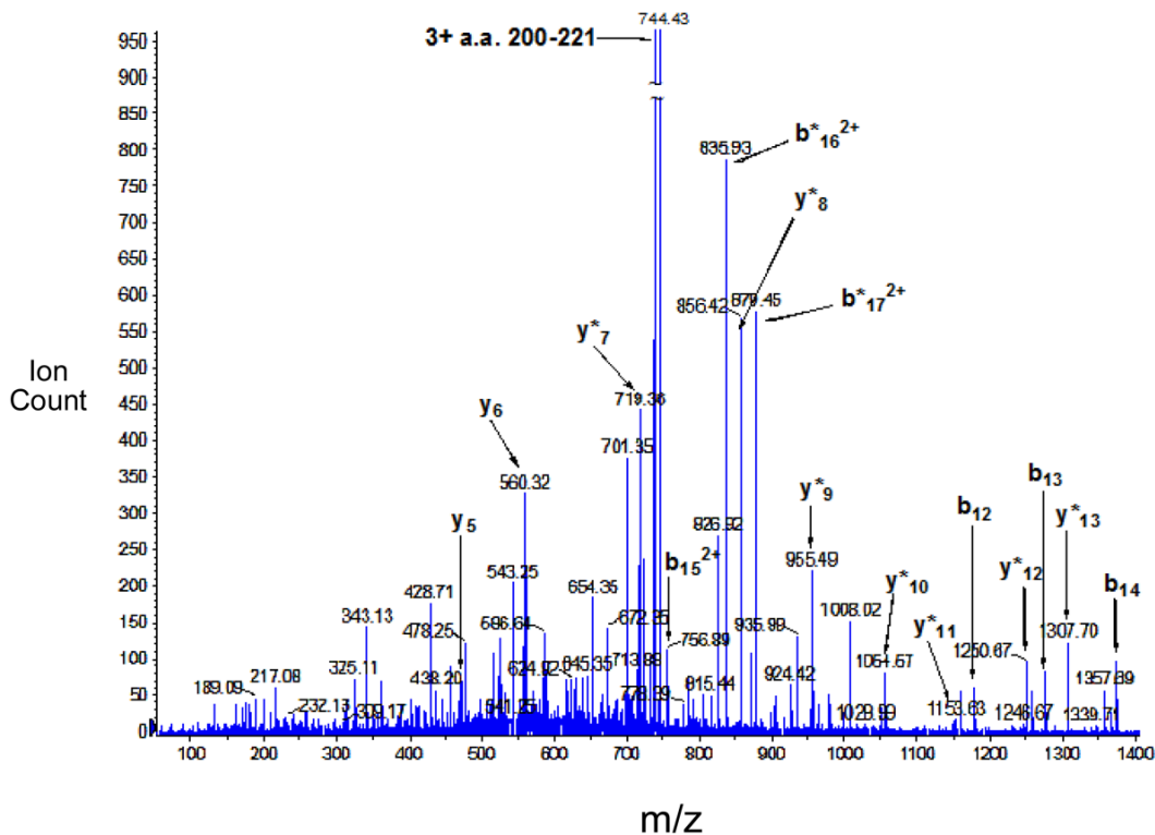
Figure 3. ESI + -MS/MS analysis of the acrolein-modified PTP1B active site tryptic fragment, E 200 SGSLSPEHGPVVVHCSAGIGR 221 . Cysteine 215 is the active site nucleophile of PTP1B. Acrolein-modified fragment ions are denoted by “*”.
