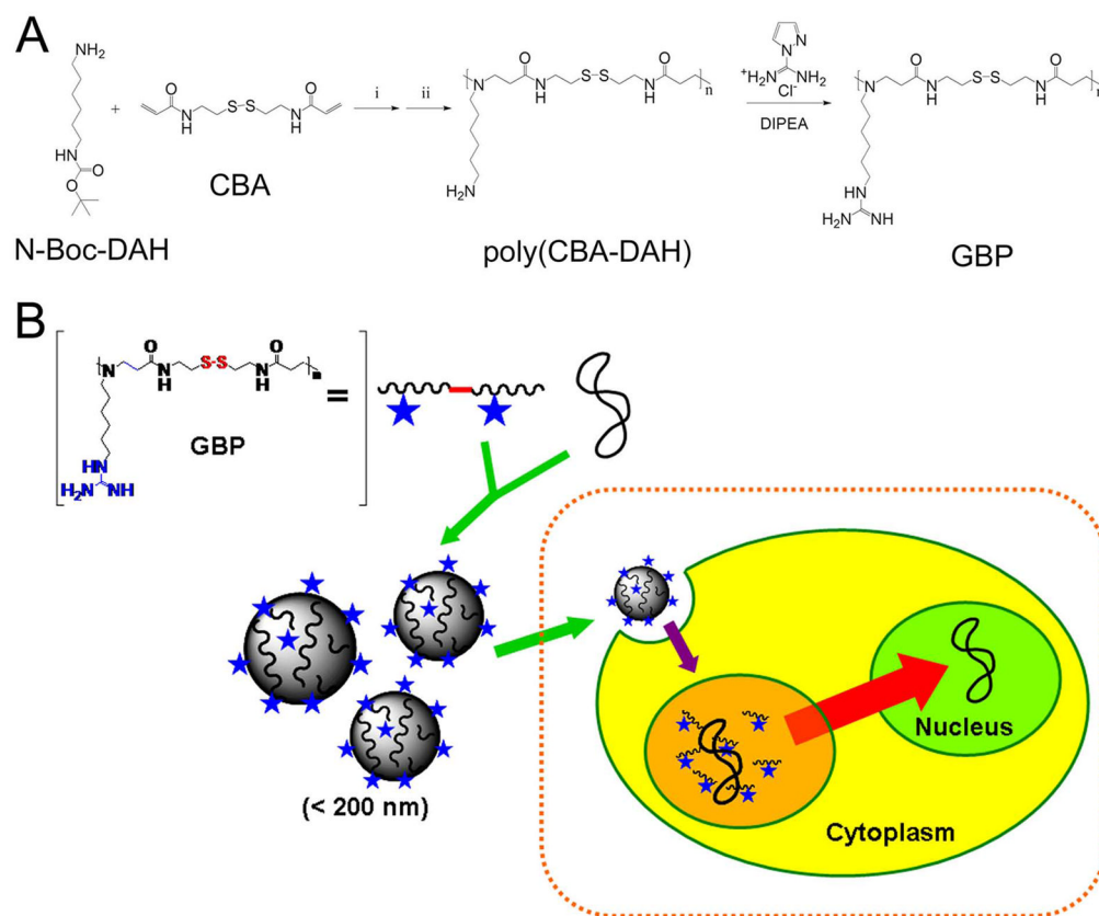
Figure 1. (A) synthetic scheme of guanidylated bioreducible polymer (GBP). i) MeOH: H 2 O = 9:1, v/v, 60 °C, 5 days, ii) TFA: triisobutylsilane: H 2 O = 95: 2.5: 2.5, v/v, 0 °C, 30 min. (B) schematic diagram of gene delivery based on GBP polyplexes.
