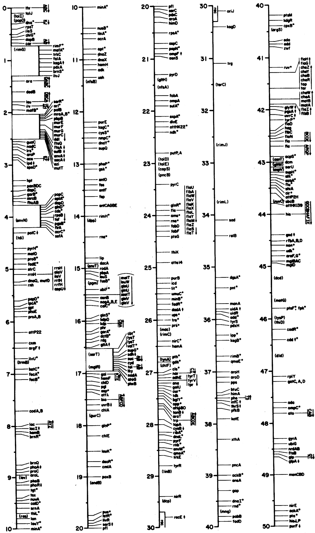
FIG. 1. Linear scale drawings representing the circular map of E. coli K-12. The time scale of 100 min, beginning arbitrarily with zero at the thr locus, is based on the results of interrupted-conjugation experiments. The genetic symbols used in this figure are defined in Table 1. Parentheses around a gene symbol indicate that the position of that marker is not well known and may have been determined only within 5 to 10 min. An asterisk
