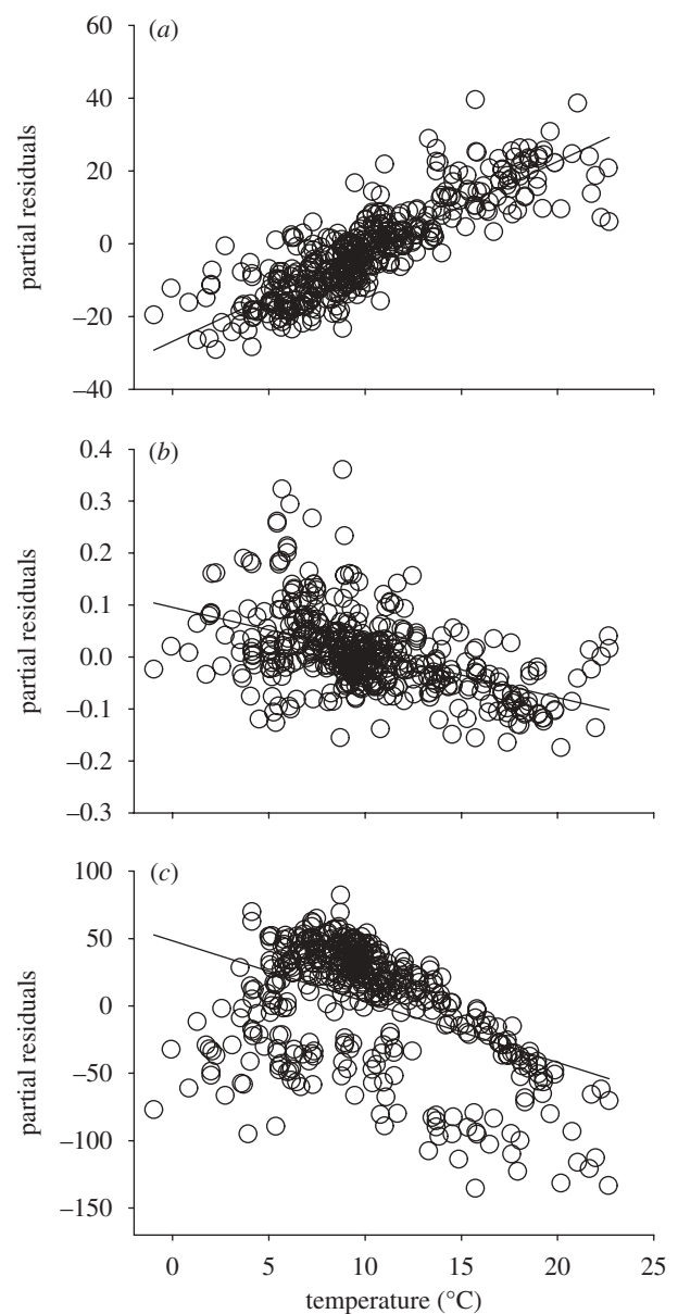
Figure 1. Observed spatial associations. Partial residuals from the OLS regression of three community attributes ((a) species richness, R^2 = 0.79 ; (b) body mass, R^2 = 0.25 ; (c) occupancy, R^2 = 0.20 ) by annual temperature for 404 North American CBC circles containing a total of 227 species. The partial residuals represent spatial trends after controlling for differences in survey effort among CBC circles. All variables used in the analysis were averaged over 1975–1977 for each CBC circle. Body mass is on a log scale.
