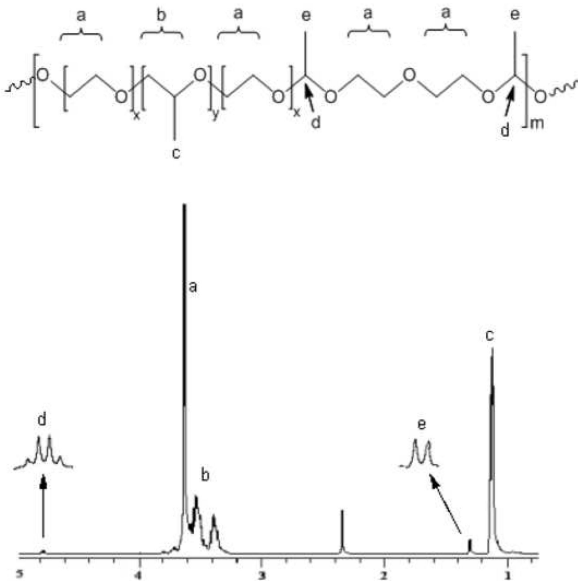
Figure 3. 1 H-NMR spectrum of MBCP-1. A quartet (d) at 4.75 ppm from acetal groups and a doublet (e) at 1.30 ppm from methyl protons of acetal groups indicated successful synthesis of MBCPs.
