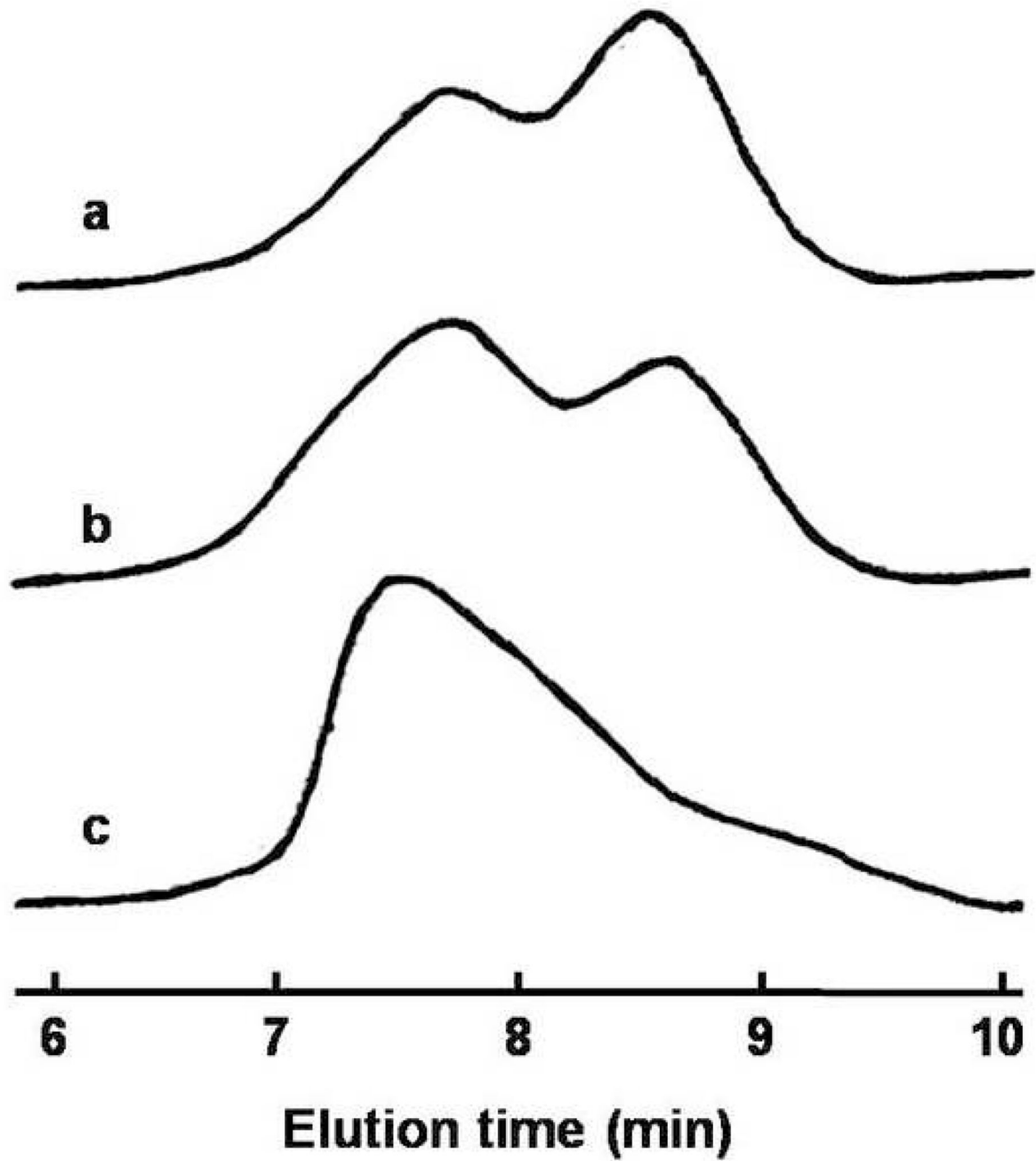
Figure 2. Gel permeation chromatograms of MBCP-2 (a) after the synthesis, (b) after the purification in aqueous NaOH and (c) after the purification in water.
