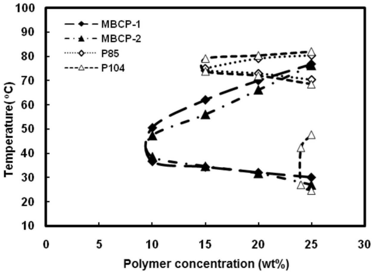
Figure 6. Phase diagrams of the aqueous solutions of Pluronic® P85, Pluronic® P104, MBCP-1 and MBCP-2 determined by the test tube inverting method.
