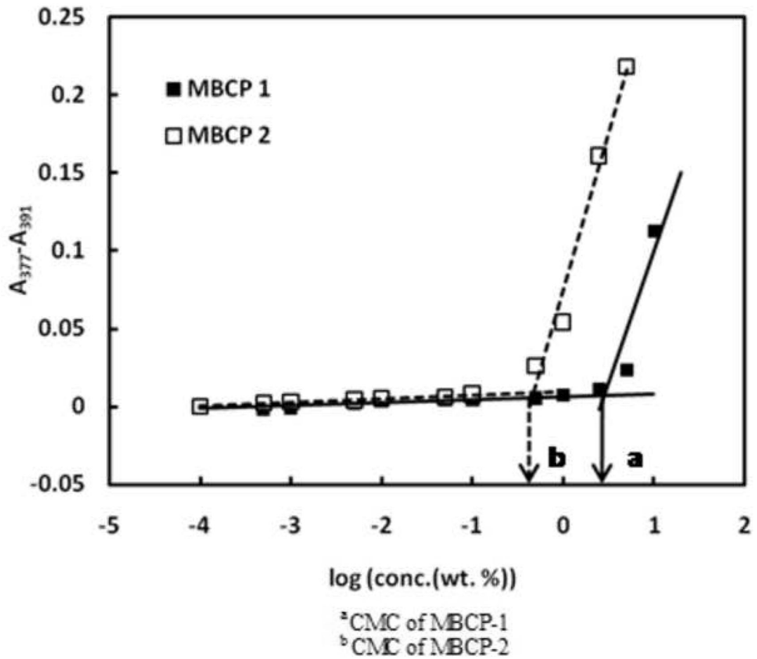
Figure 4. Determination of CMC of the synthesized MBCPs by the dye solubilization. The difference in the absorbance of DPH at 377 and 391nm was plotted on vertical axis. The cross-section point of the two exponential lines was defined as the CMC. The CMCs of MBCP-1 and MBCP-2 were 2.854 ( \pm 0.030 ) wt% and 0.485 ( \pm 0.009 ) wt%, respectively.
