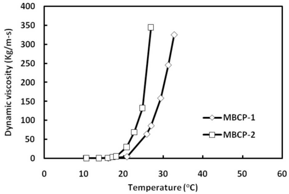
Figure 7. Determination of dynamic viscosity changes of MBCP-1 and MBCP-2 aqueous solutions as a function of temperature using falling ball method. The polymer concentration was 25 wt%. The MBCP solutions were equilibrated for 20 minutes at each temperature.
