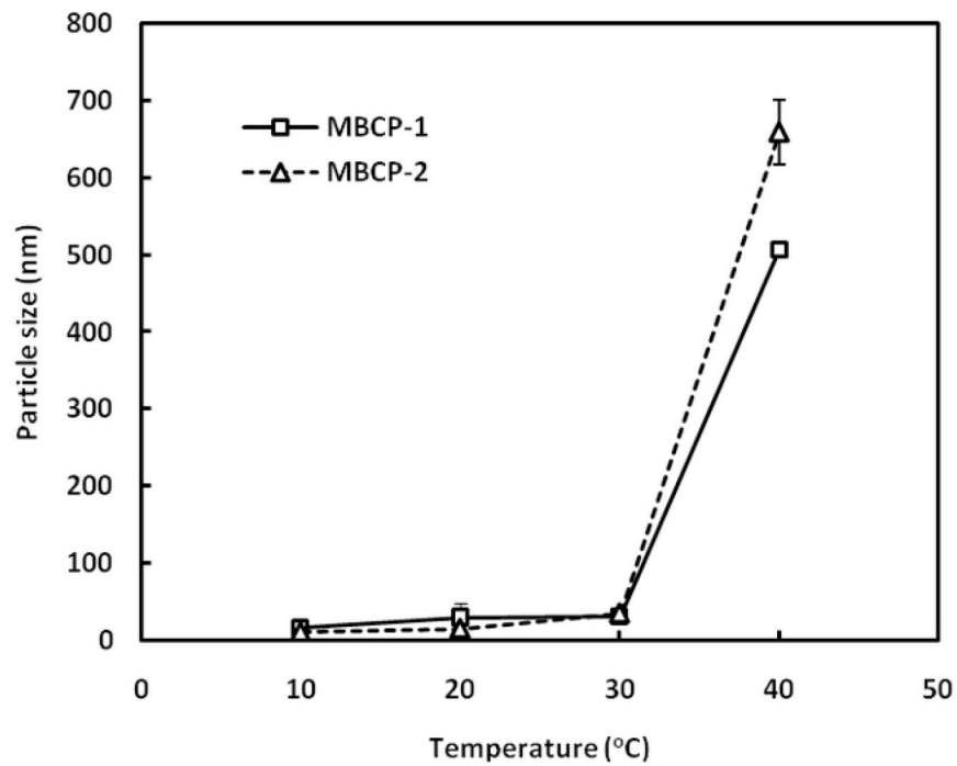
Figure 8. Determination of micellar size changes of MBCP-1 and MBCP-2 using dynamic light scattering. The micellar size changes were measured as a function of temperature. The polymer concentration was 4% w/v. The results represent the mean \pm SD for n=3 .
