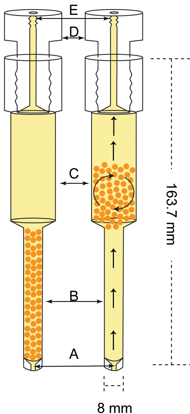
Fig. 1. The CEC bioreactor. On the left, the pump is off and the encapsulates are settled. On the right, the pump is on and the encapsulates circulate at a steady state in the upper chamber. A: tubing inlet, B: NMR detection region, C: circulation chamber, D: adjustable threaded cap, E: fitting inlet. Orange circles represent encapsulates containing E. coli cells.
