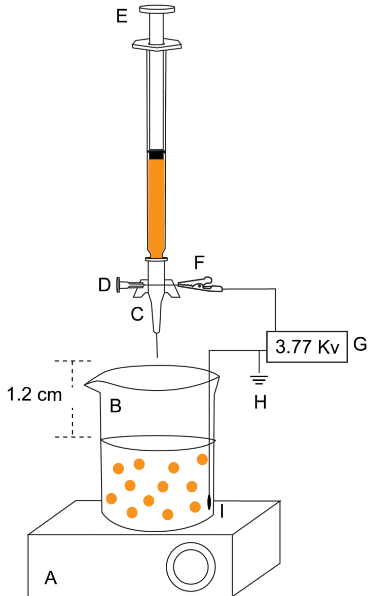
Fig. 7. Schematic of the electrostatic encapsulation device. A: stir plate, B: beaker containing 150 mM \text{CaCl}_2 , C: anion catheter, D: needle, E: insulin syringe, F: alligator clip (connects the positive power supply terminal to the needle) G: high voltage power supply, H: ground, I: negative end
