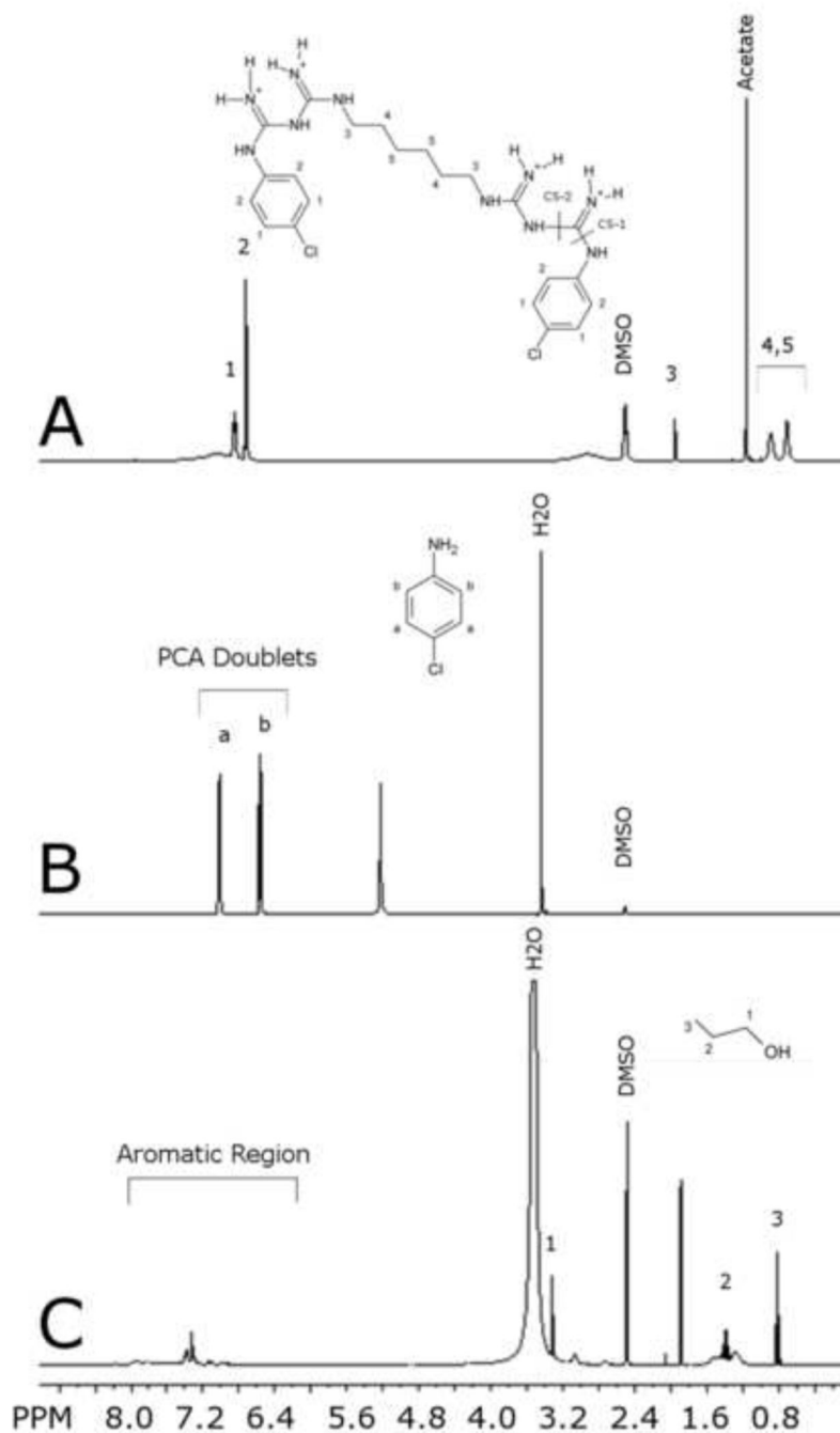
Figure 1. ^1\text{H} NMR spectrum of (A) chlorhexidine acetate with characteristic peaks at 6.85 ppm and 6.71 ppm (labels 1–5 correspond to labeled chemical structure of chlorhexidine and cleavage sites are labeled CS-1 and CS-2) (B) p-chloroaniline with characteristic peaks at 7.01 ppm and 6.56 ppm (labels a and b correspond to labeled chemical structure of PCA). (C) Reaction precipitate sampled at 60 minutes with n-propanol added at 0.4 mg/ml as an internal standard (labels 1–3 corresponding to labeled chemical structure of n-propanol). All spectra were taken with 400-MHz Varian NMR System at 25°C, acquiring 32 scans, in d_6 -DMSO solvent.
