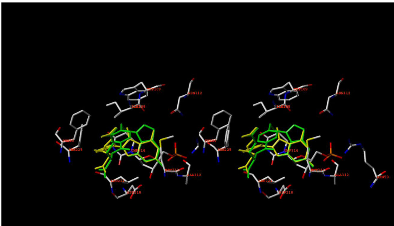
Figure 3. Stereoview 5 (yellow) superimposed on pemetrexed (green) in the X-ray crystal structure of pemetrexed in human TS (PDB: 1JUU) 25 using SYBYL 8.1.
