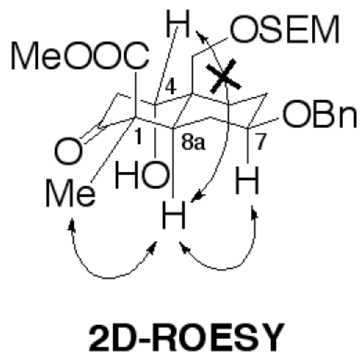
Figure 4. The relative stereochemistry of compound ( 15 ) as determined by 2D-ROESY experiment.
