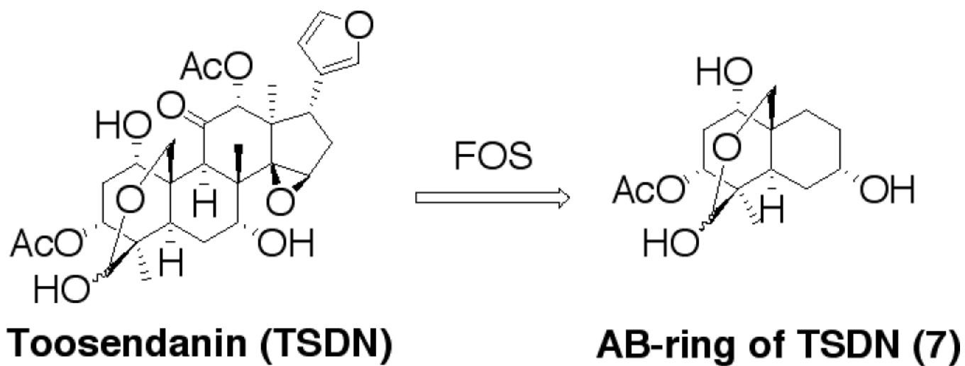
Figure 3. AB-ring of toosendanin (7).
