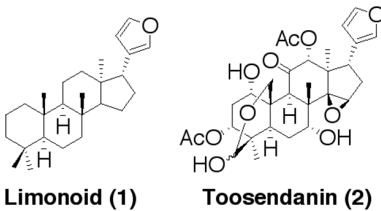
Figure 1. General structures of limonoid (1) and toosendanin (2).
