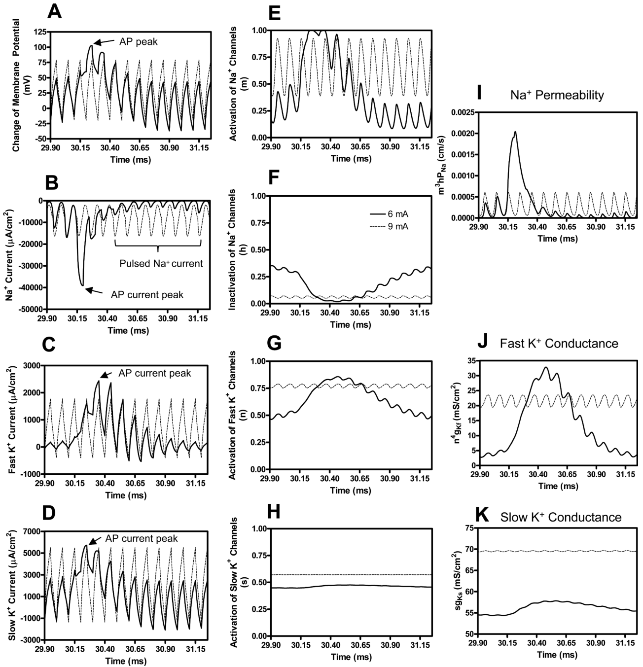
Fig. 7. Mechanism underlying the disappearance of the repetitive firing as shown in Fig. 2C-D when the HFB stimulation intensity increases from 6 mA to 9 mA. No test pulse is applied in this figure. Axonal activities at the node under the electrode are shown in A-H. The legend in F indicates the HFB stimulation intensity. HFB stimulation frequency: 10 kHz; Axon diameter: 2 \mu\text{m} . AP – action potential. Note: the AP duration lasts for several cycles of the HFB stimulation.
