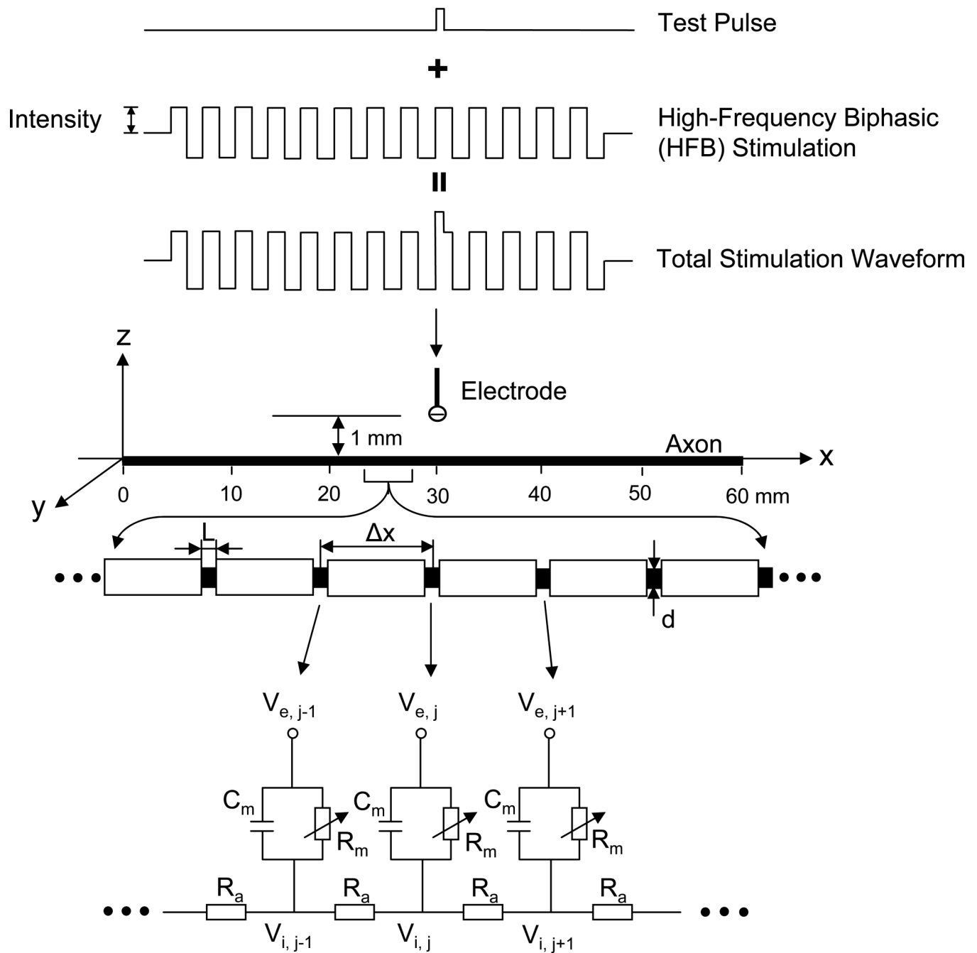
Fig. 1. Myelinated axonal model used to simulate the modulation of axonal excitability by high-frequency biphasic (HFB) electrical stimulation. The inter-node length \Delta x = 100d ; d is the axon internal myelin diameter. L is the nodal length. Each node is modeled by a resistance-capacitance circuit based on SRB model. R_a : inter-nodal axoplasm resistance; R_m : nodal membrane resistance; C_m : nodal membrane capacitance; V_{i,j} : intracellular potential at the j^{\text{th}} node; V_{e,j} : extracellular potential at the j^{\text{th}} node.
