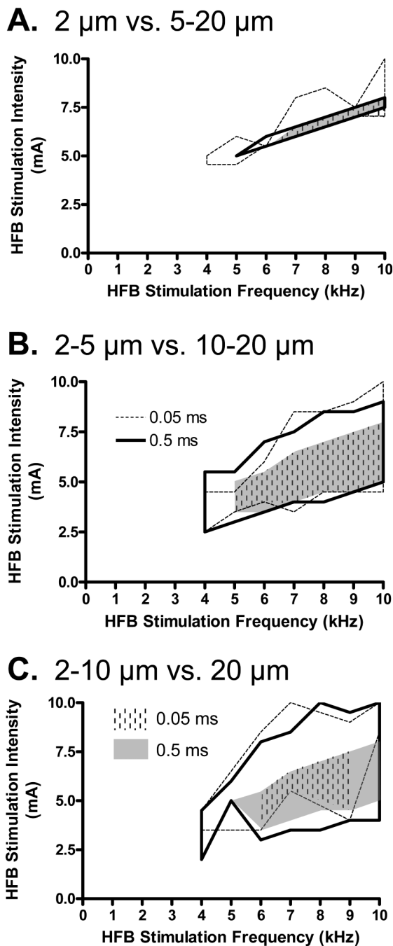
Fig. 5. HFB stimulation frequencies, intensities, and test pulse widths for selectively activating different groups of smaller axons without activating larger axons: A. 2 \mu\text{m} vs. 5-20 \mu\text{m} ; B. 2-5 \mu\text{m} vs. 10-20 \mu\text{m} ; C. 2-10 \mu\text{m} vs. 20 \mu\text{m} . The legends in B and C indicate different test pulse widths which apply to all graphs. The stimulation parameters enclosed by thick or dashed lines are suitable for activating the small axons without activating the large axons. The grey or dashed areas indicate the regions where the small axons fire action potentials repetitively.
