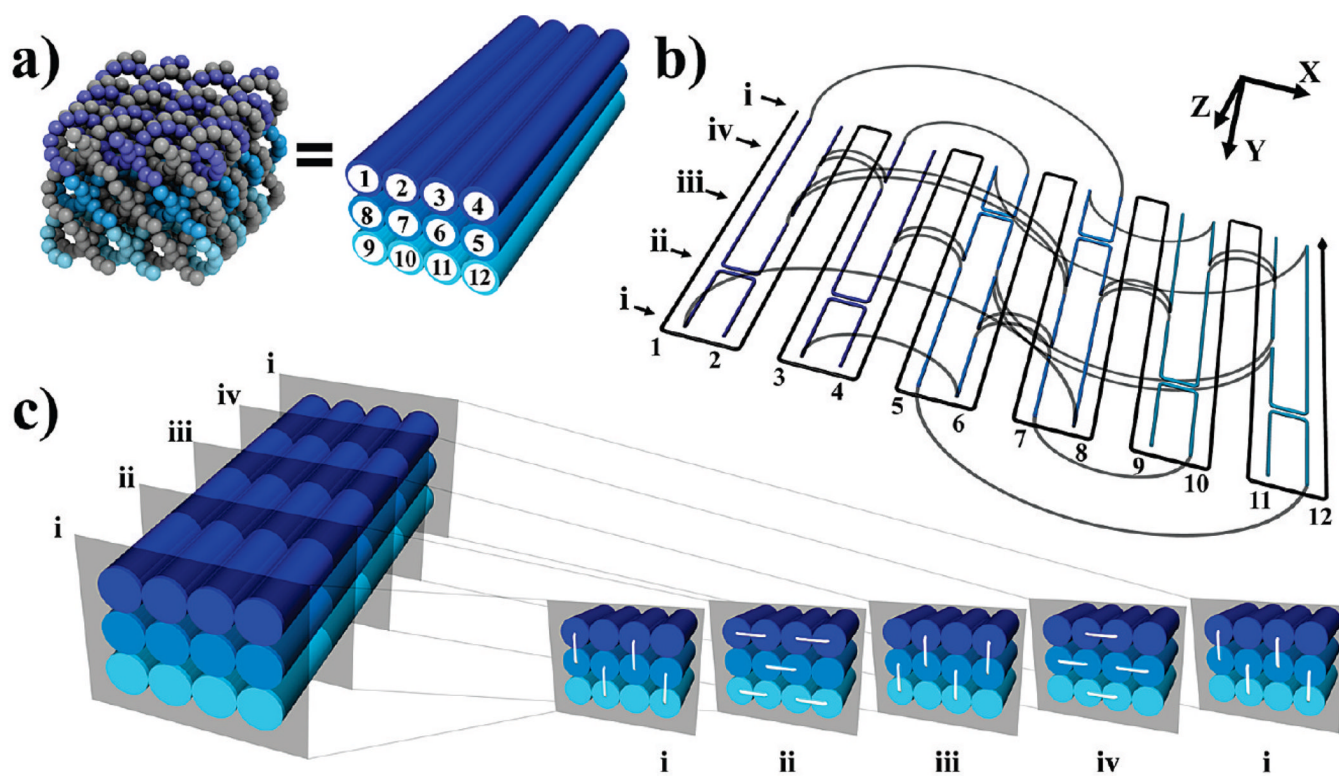
Figure 1. Design of multilayer three-dimensional DNA origami on a square lattice. (a) Helical DNA model of the 3D origami square-lattice structure. The scaffold strand is in gray and the staple strands are in three shades of blue. This model is equivalent to the cylinder model shown on the right. Each cylindrical rod represents one DNA double helix. The numbers labeled at the helical ends indicate the order of the scaffold-strand segments that thread through the helices. (b) Layout and connectivity of the scaffold strand (gray) and the staple strands (colored), in an unfolded two-dimensional scheme of the target shape. Phosphate linkages that form crossovers between adjacent helices are shown as curved lines. The positions of the crossover points of the staple strands are labeled from i to iv, which are spaced apart at 8-bp intervals. (c) Three-dimensional cylinder model of the folded target shape. The square-lattice arrangement of parallel helices is revealed in cross-sectional slices (i–iv) that are parallel to the xy -plane spaced at 8-bp intervals and repeating every 32 bp. Staple crossovers are shown as white lines linking two adjacent helices at each cross section.
