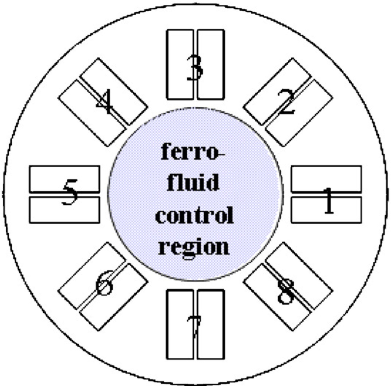
Fig. 3. Current model setup. Eq. (1) is solved everywhere in the simulation domain which includes the 8 controlled magnets and the inner domain where ferrofluid transport takes place (Eqs. (1) and (2)).
