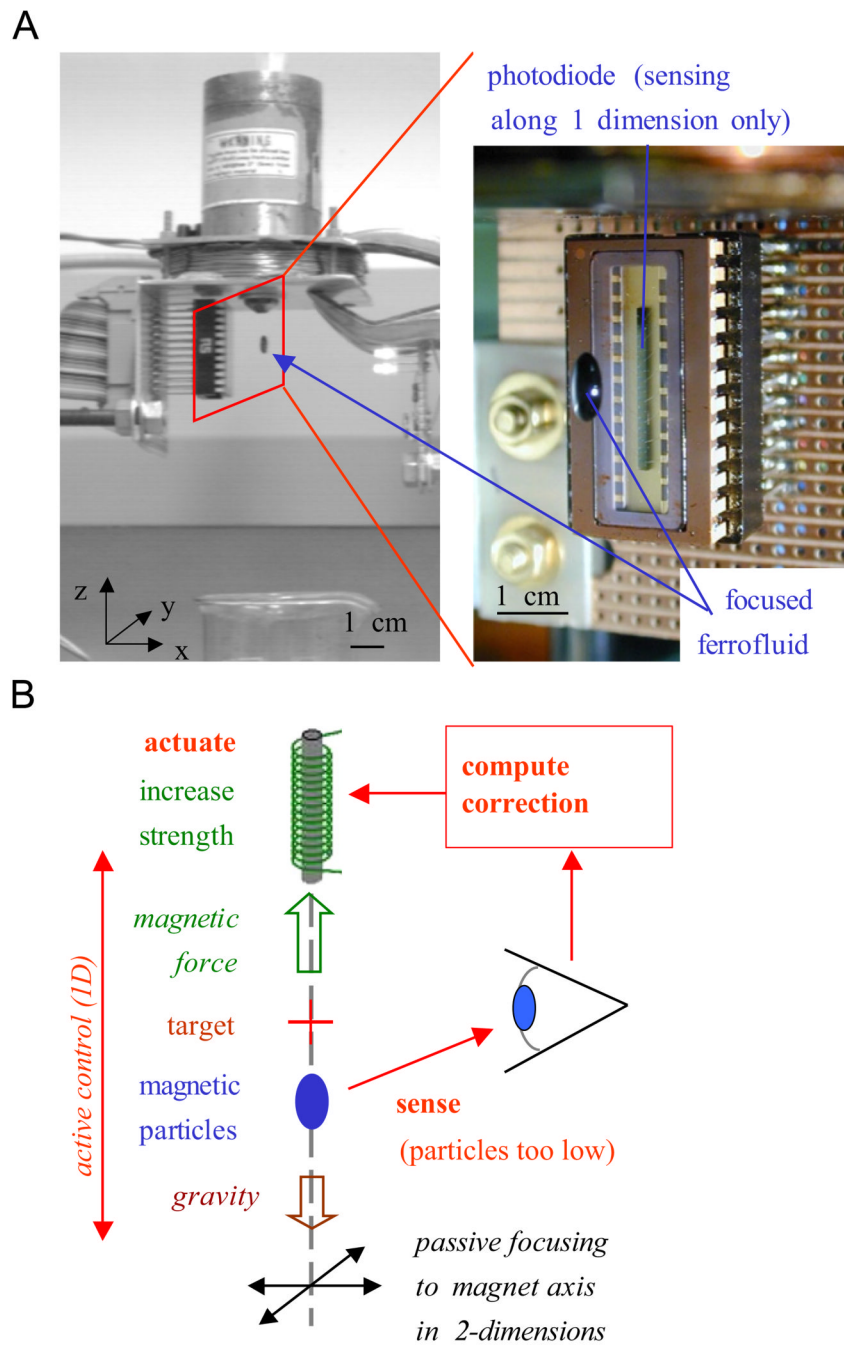
Fig. 2. Using dynamic actuation it is possible to trap ferrofluid at a distance from a single electromagnet. (A) The controlled magnet applies a field of \sim 0.02 T and holds a 0.8mm drop of ferrofluid at a 1cm distance. The zoom shows the trapped fluid and the photodiode infrared sensor, which senses the location of the fluid along the z -axis only. (B) Feedback control loop. Focusing in x and y does not require feedback, the particles are passively attracted to the magnet axis. Active control occurs only along z , when the drop is too low the magnet strength is increased to raise it (and vice versa).
