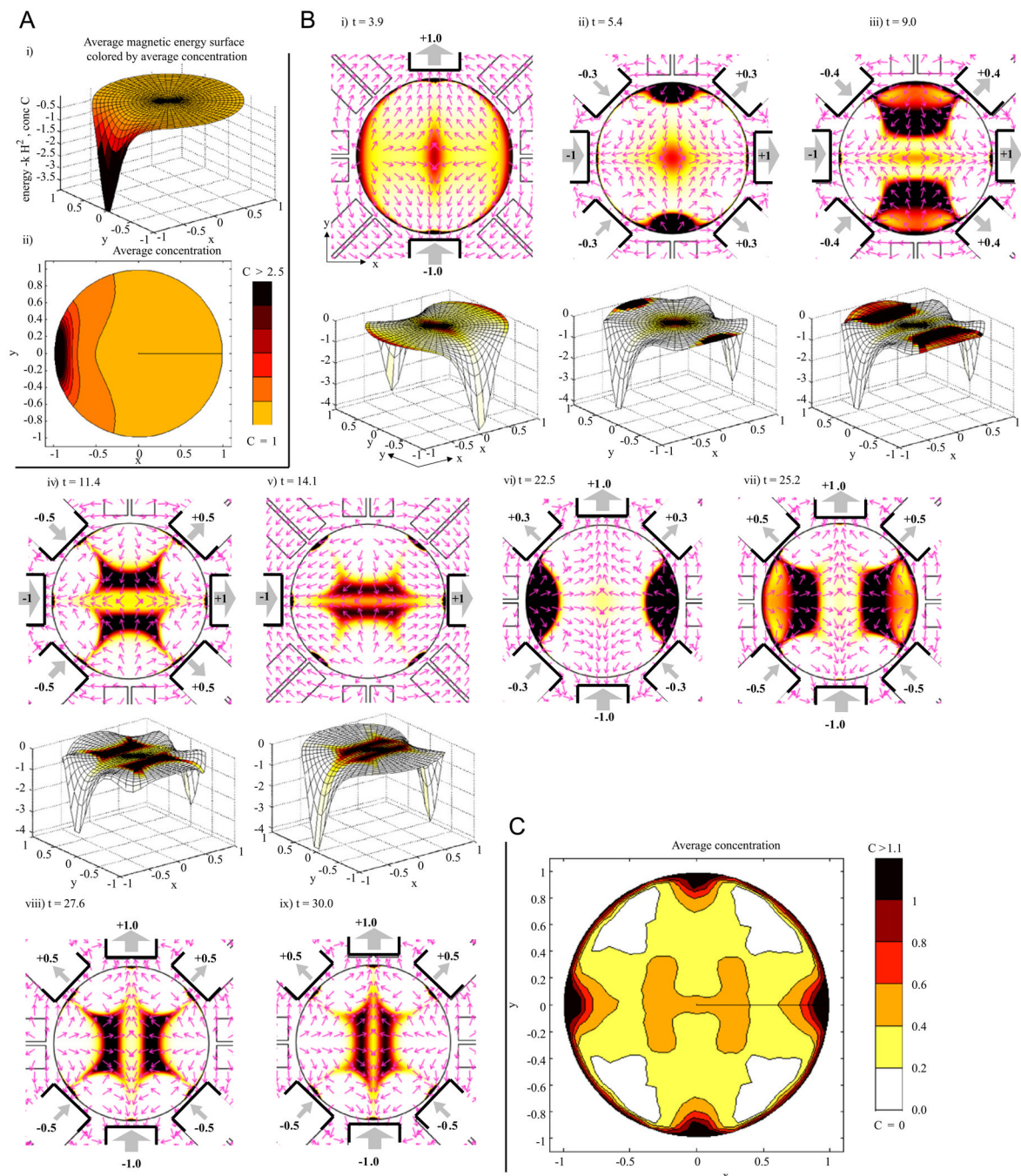
Fig. 4. (A) Constant actuation: ferrofluid transport due to turning on the 5th (far left) magnet. (i) The magnetic energy surface U = -kH^2 is plotted along the z -axis to show ferrofluid flowing downhill along the force directions F = -\nabla U with the resulting averaged concentration shown by the coloring here and in sub-panel (ii). (B) Dynamic control: magnets are now turned on and off to transport ferrofluid to the center. The first 5 sub-panels show ferrofluid concentration and magnetic actuation with the corresponding magnetic energy surfaces. Energy surfaces for the last 4 panels (not shown) are 90^\circ flips of the ones shown (see the main text). Coloring denotes concentration (scale bar same as in C). On magnets are illustrated by heavy black lines with weighted thick gray arrows and numbering showing magnet strength and orientation
