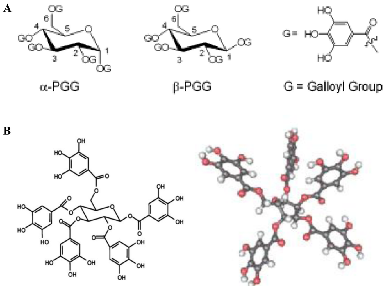
Fig. 1. A. Sterical configuration of \alpha -PGG and \beta -PGG (ref. 3) B. Structure and 3D model of \beta -PGG (ref. 7)
