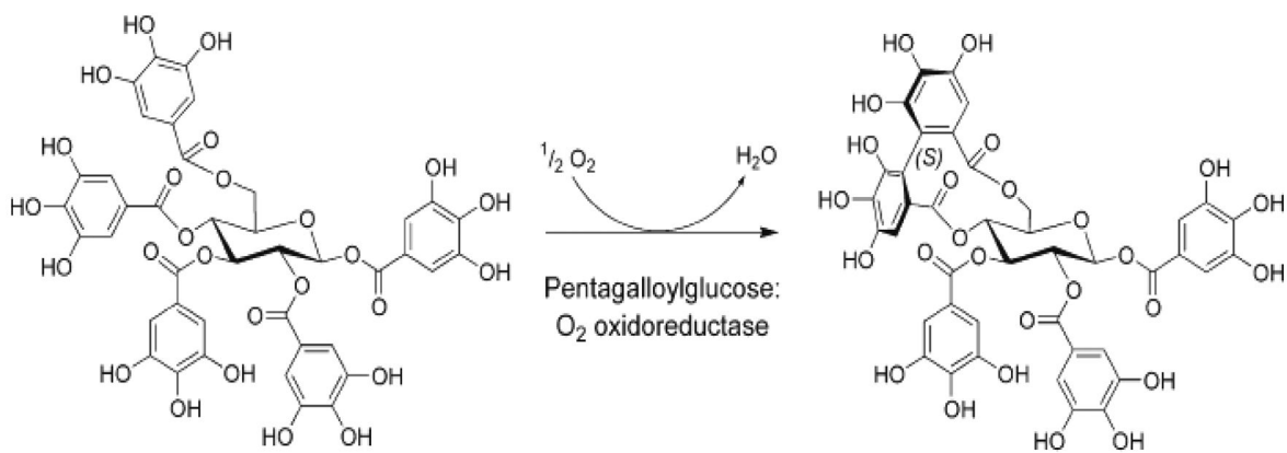
Fig. 2. An example of oxidoreductase-catalyzed the intra-molecular oxidative cross-linking reactions (ref 13).
