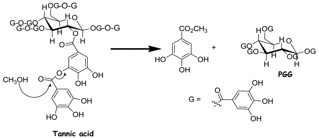
Fig. 3. Methanolysis of tannic acid to yield PGG under weak acidic condition (ref. 21).
