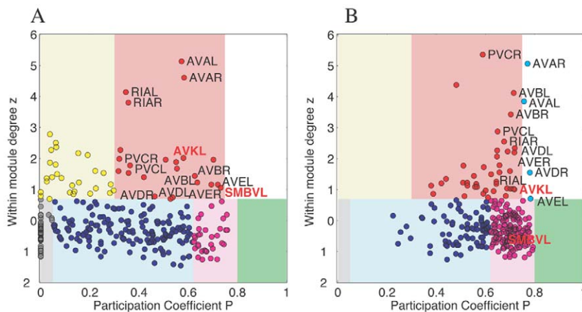
Figure 9. The role of individual neurons according to their intra- and inter-modular connectivity. (A) The within module degree z -score of each neuron in the empirical neuronal network is shown against the corresponding participation coefficient P . The within module degree measures the connectivity of a node to other nodes within its own module, while the participation coefficient measures its connectivity with neurons in the entire network. (B) The corresponding result for a randomized version of the C. elegans network where the degree of each neuron is kept unchanged is also shown. Neurons belonging to the different regions in the P-z space are categorised as: (gray) R1: “ultraperipheral nodes”, i.e., nodes with all their links within their module, (blue) R2: “peripheral nodes”, i.e., nodes with most links within their module, (pink) R3: “nonhub connector nodes”, i.e., nodes with many links to other modules, (green) R4: “nonhub kinless nodes”, i.e., nodes with links homogeneously distributed among all modules, (yellow) R5: “provincial hubs”, i.e., hub nodes with the vast majority of links within their module, (red) R6: “connector hubs”, i.e., hubs with many links to most of the other modules, and (white) R7: “global hubs”, i.e., hubs with links homogeneously distributed among all modules. The neurons occurring as connector hubs are identified in the figure. Most of these neurons occur in different functional circuits indicating the close relation between functional importance and connectivity pattern of individual neurons. In addition, the neurons AVKL and SMBVL which are predicted to be functionally important are separately marked.
