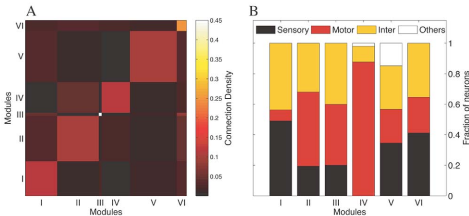
Figure 2. Modular interconnectivity and decomposition according to neuron type. (A) Matrix representing the average connection density between neurons occurring within modules and those in different modules. The figure indicates that neurons within a module are densely interconnected compared to the overall connectivity in the network. (B) The modules are decomposed according to the different neuron types comprising them. The figure shows that the modules are not simply composed of a single type of neuron. doi:10.1371/journal.pone.0009240.g002
