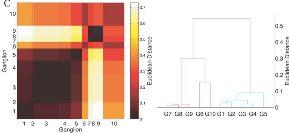
Figure 4. Modular decomposition of neurons in different ganglia. (A) Neurons belonging to different ganglia are decomposed according to their modular membership. The height of each bar in the histogram corresponds to the overlap between the ganglia and the modules, calculated as the fraction of neurons that are common to a particular ganglion and a specific module. (B) The matrix representing the average modular distance between the different ganglia, as calculated from the modular decomposition spectrum of each ganglion. The corresponding dendrogram indicates the closeness between different ganglia in the abstract 6-dimensional “modular” space. (C) The matrix of physical distances between the ganglia is shown for comparison with (B), calculated as the average distance between neurons belonging to the different ganglia. The corresponding dendrogram indicates the closeness between ganglia according to the geographical nearness of their constituent neurons in the nematode body. The difference indicates that the ganglia which are geographically close may not be neighbors in terms of their modular spectra. doi:10.1371/journal.pone.0009240.g004
