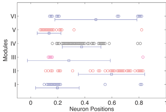
Figure 3. Neuronal layout of the worm indicating cell body positions of each neuron. The position of neuronal cell bodies along the longitudinal axis of the C. elegans body plan is shown, with the vertical offset and color indicating the module to which a neuron belongs. The mean and standard deviation of neuronal positions for each module is also indicated, suggesting relative absence of spatial localization in the modules.
