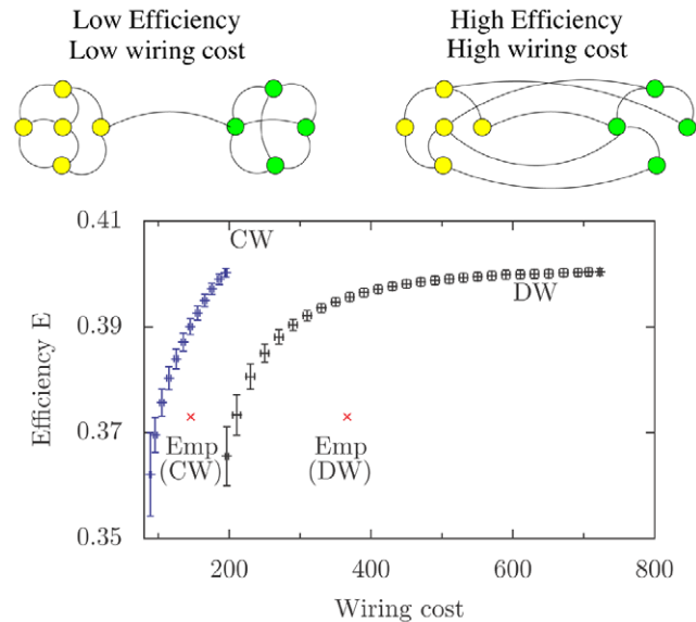
Figure 6. Trade-off between wiring cost and communication efficiency in the network. The variation of communication efficiency, E , as a function of the wiring cost, defined using either the “dedicated-wire” model (DW) or the “common-wire” model (CW), in the ensemble of random networks with degree sequence identical to the C. elegans neuronal network. The trend indicates a trade-off between increasing communication efficiency and decreasing wiring cost. The corresponding values for the empirical network are indicated by crosses for both DW and CW. The schematic figures shown above the main panel indicate the type of networks obtained in the limiting cases when only one of the two constraints are satisfied. In both curves, error bars indicate the standard deviations calculated for 10^3 random realizations. We observe that the empirical network is suboptimal in terms of wiring cost and communication efficiency, suggesting the presence of other constraints governing the network organization. doi:10.1371/journal.pone.0009240.g006
