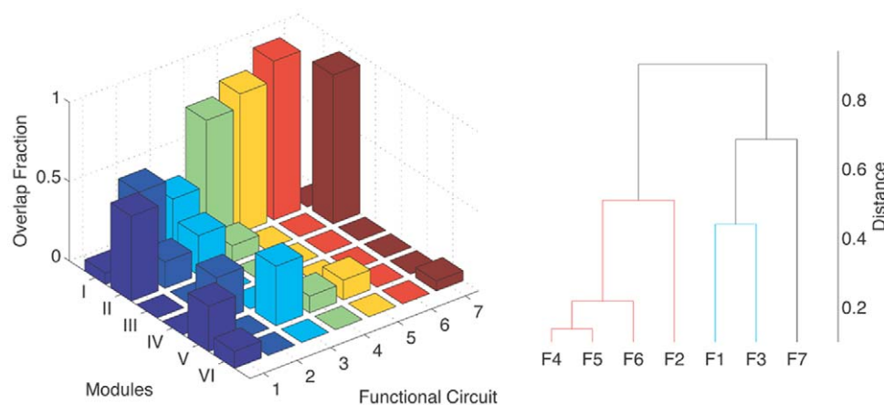
Figure 8. Modular decomposition of neurons in different functional circuits. Neurons belonging to different functional circuits are decomposed according to their modular membership. The height of each bar in the histogram corresponds to the overlap between the modules and functional circuits (F1) mechanosensation, (F2) egg laying, (F3) thero-taxis, (F4) chemosensation, (F5) feeding, (F6) exploration and (F7) tap withdrawal. The overlap is measured in terms of the fraction of neurons common to a particular functional circuit and a specific module. The corresponding dendrogram represents the closeness between different functional circuits in the abstract 6-dimensional “modular” space. doi:10.1371/journal.pone.0009240.g008
