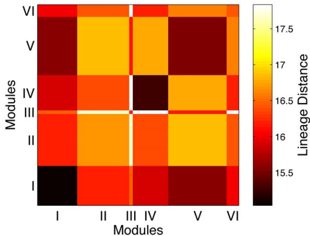
Figure 5. Lineage distance between modules. The matrix representing the average lineal distance between neurons occurring within the same module and those belonging to different modules. The figure indicates that neurons occurring in the same module have only a slightly lower lineal distance as compared to that between neurons occurring in different modules. doi:10.1371/journal.pone.0009240.g005
