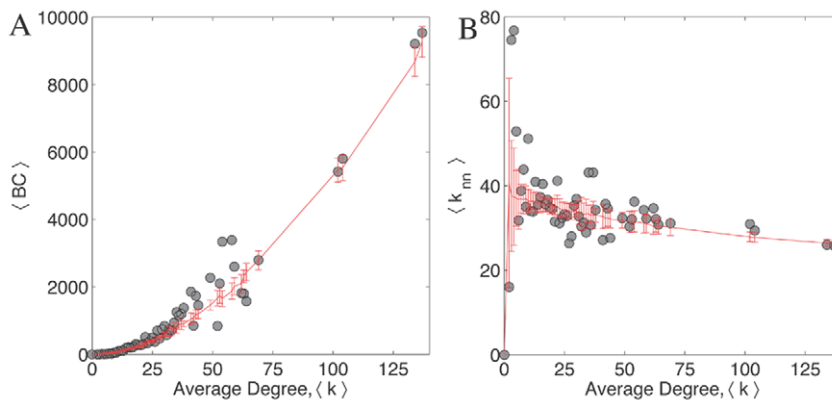
Figure 7. Betweenness centrality and the average nearest neighbor degree as a function of the total degree of network. (A) The average betweenness centrality, \langle BC \rangle , and (B) the average nearest neighbor degree, \langle k_{nn} \rangle of each node as a function of its total degree, \langle k \rangle = \langle k_{in} + k_{out} \rangle . Betweenness centrality is a measure of how frequently a particular node is used when a signal is being sent between any pair of nodes in the network using the shortest path. In case of the Internet, BC of nodes increases with its degree which is sought to be linked with its information transport property. In C. elegans , although BC increases with degree, this increase is not significant when compared to the randomized version of the network. In the case of the relation between the average connectivity of nearest neighbors of a node with its total degree k , we note that for both the Internet and protein interaction network, k_{nn} decreases with k as a power law. This means that low connectivity nodes have high degree nodes as their neighbors and vice-versa. However, in the case of C. elegans , this relation is not very apparent and insignificant in comparison with the randomized version of the network. In both figures, error bars indicate the standard deviations calculated for 10^3 random realizations. These results suggest that the C. elegans network forms a class distinct from the class of networks optimized only for signal propagation. doi:10.1371/journal.pone.0009240.g007
