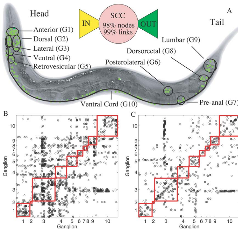
Figure 1. Neuronal position and connectivity in the somatic nervous system of the nematode C. elegans indicating the different ganglia. (A) Schematic diagram of C. elegans , indicating the different ganglia. (Inset) Schematic representation of connectivity between the neurons, partitioned into a strongly connected component (SCC), an in-component (IN), and an out-component (OUT). A directed path exists from any neuron in IN to any neuron in OUT through neurons in SCC, all of whose members can be reached from each other. The large SCC suggests that it is possible to transfer signals between almost all neurons of the network. The IN and OUT components have only 1.5% and 0.5%, respectively, of the 279 connected neurons in the somatic nervous system. (B, C) The connectivity matrix corresponding to the (B) Synaptic and (C) Gap-junctional connections between the somatic system neurons. In all figures, the partition symbols correspond to (G1) Anterior, (G2) Dorsal, (G3) Lateral, (G4) Ventral, (G5) Retrovesicular, (G6) Posterolateral, (G7) Preanal, (G8) Dorsorectal and (G9) Lumbar ganglion, and (G10) the Ventral cord. doi:10.1371/journal.pone.0009240.g001
