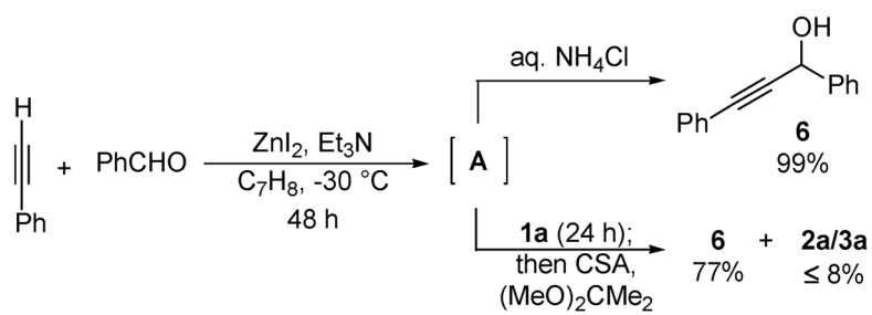
Scheme 2. Mechanistic Study
