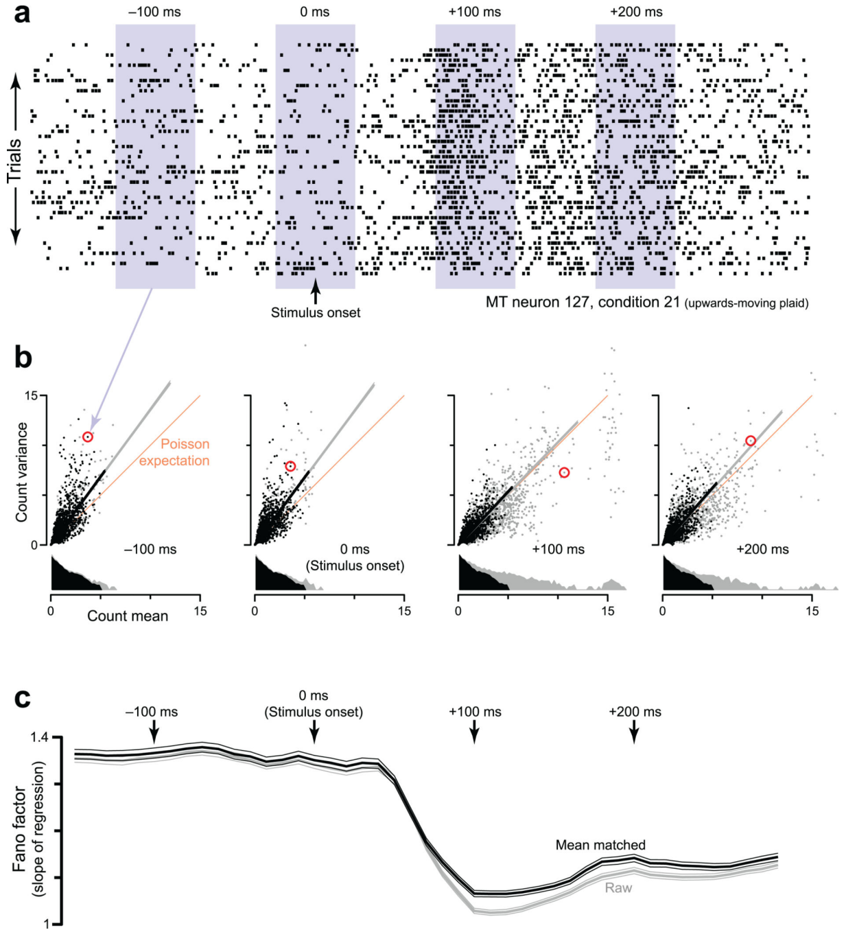
Figure 4. Illustration of how the mean-matched FF was computed. Data are from the MT-plaids dataset. a. Spike rasters for the 46 trials (one per line) recorded from one MT neuron (127) for one stimulus condition (upwards-moving plaid). Shaded areas show 4 locations of the sliding window, which moved in 10 ms increments. For each window location, the spike count was computed for each trial. The mean and variance (across trials) of that count then contributed one data-point to the subsequent analysis ( next panel ). b. The FF was computed based on scatterplots of the spike-count variance versus mean. Each scatterplot corresponds
