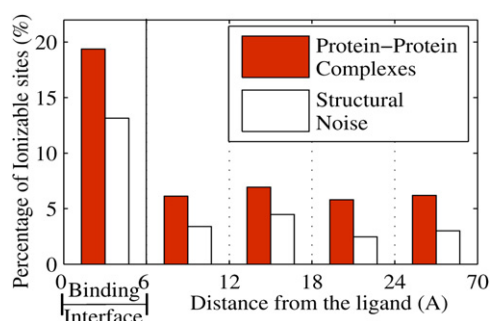
FIGURE 3 Distance distribution of ionizable residues with substantial pK change in the biologically relevant pH range. (Solid red bars) Overall procedure in protein-protein complexes; (open bars) false-positive pK changes due to structural noise. The percentage in each region is relative to the number of residues located in that region.
