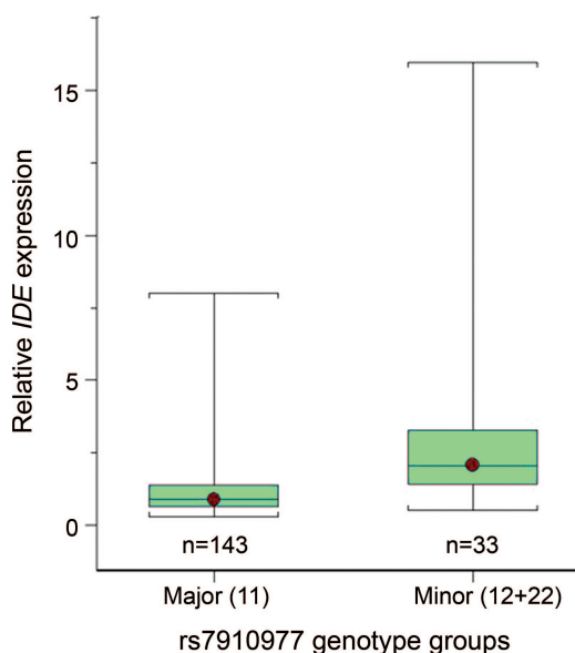
Figure 1 Relative IDE expression levels by rs7910977 genotypes
