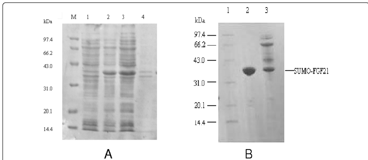
Figure 3 SDS-PAGE analysis of expression and purification of SUMO-FGF21. Bacterial containing pET-SUMO-FGF21 were induced by IPTG for 3 h or 4 h at 37°C in Figure 3A. The results from the different treatments are shown here. M: protein molecular weight markers; Lane 1: the supernatant of BL21 (DE3) containing pET-SUMO-FGF21 without IPTG; Lane 2: the supernatant of BL21 (DE3) containing pET-SUMO-FGF21 induced with 1 mM IPTG for 3 h; Lane 3: the supernatant of BL21 (DE3) containing pET-SUMO-FGF21 induced with 1 mM IPTG for 4 h; Lane 4: the precipitation of BL21 (DE3) containing pET-SUMO-FGF21 induced with 1 mM IPTG for 4 h. After recombinant bacteria were treated by sonication and centrifugation, the supernatants were loaded on a DEAE sepharose FF and Ni-NTA orderly. The purification results for SUMO-FGF21 are shown in the Figure 3B. Lane1: protein molecular weight marker, Lane2: purified SUMO-FGF21 eluted from Ni-NTA column; Lane3: SUMO-FGF21 eluted from DEAE sepharose FF column.
