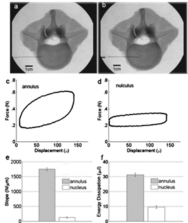
FIG. 2. Demonstration of the ability of the TDI to distinguish between the annulus and nucleus of a human intervertebral disk. (a) X-ray image of transverse view of a cadaver lumbar motion segment L12 with test probe located in annulus. (b) Similar view with probe centered in the nucleus. (c) Force vs displacement curve measured by the TDI during a cyclic load cycle (4 Hz) in the annulus. (d) Force vs displacement curve measured in the nucleus. Note that the annulus is much stiffer (higher slope) and dissipates more energy (higher area enclosed by the curve). (e) Histogram comparing the average least-squares slope for ten cycles in the annulus vs in the nucleus. (f) Histogram comparing the average energy dissipation for ten measurements in the annulus vs in the nucleus ( 31.8 \pm 1.1\ \mu\text{J} vs 9.7 \pm 0.6\ \mu\text{J} ; p < 0.01 ). The error bars indicate standard deviation for the ten measurements within the annulus and within the nucleus in the disk.
