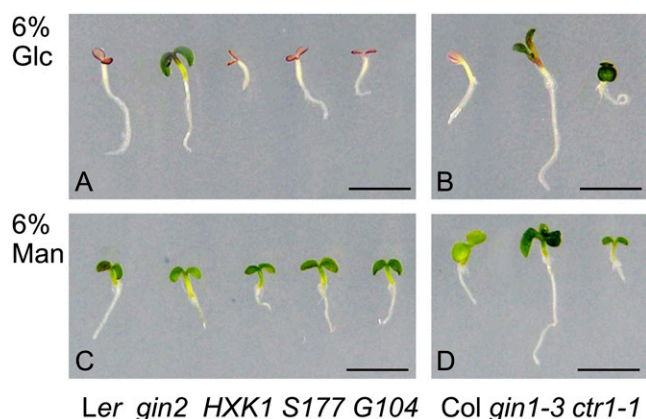
Figure 1. Glc-insensitive phenotype of gin2 displayed on a high 6% Glc MS medium. A, The gin2 mutant (5 d) shows insensitivity to Glc-mediated developmental arrest on a 6% Glc plate (1× MS) under constant light. B, The gin1 and ctr1 mutants show an insensitive phenotype to 6% Glc (1× MS). C and D, Similar seedling growth was observed on 6% mannitol (Man) MS medium. Scale bars, 5 mm. [See online article for color version of this figure.]
