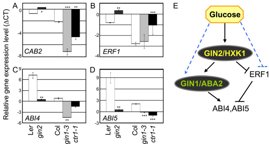
Figure 3. Low Glc-dependent gene regulation. A, gin2 mutants are insensitive to Glc repression of CAB2 (At1g29920). B, ERF1 (At3g23240) expression is repressed by low Glc signaling in wild type ( Landsberg erecta , Columbia), gin1 , and ctr1 , but not in gin2 . C and D, ABI4 (At2g40220) and ABI5 (At2g36270) expression is induced by low Glc signaling in wild type, but not in gin1 , gin2 , and ctr1 . Values are normalized based on those obtained from seedlings grown on mannitol and means of triplicate measurements with error bars are shown. The experiments were repeated twice with similar results. Asterisks over bars indicate differences between wild type and mutants with statistical significance at * P < 0.05 , ** P < 0.01 , and *** P < 0.001 ( t test). E, A model of HXK1-dependent (solid line) pathways in high and low Glc signaling and HXK1-independent (dashed line) pathways in high Glc signaling. [See online article for color version of this figure.]
