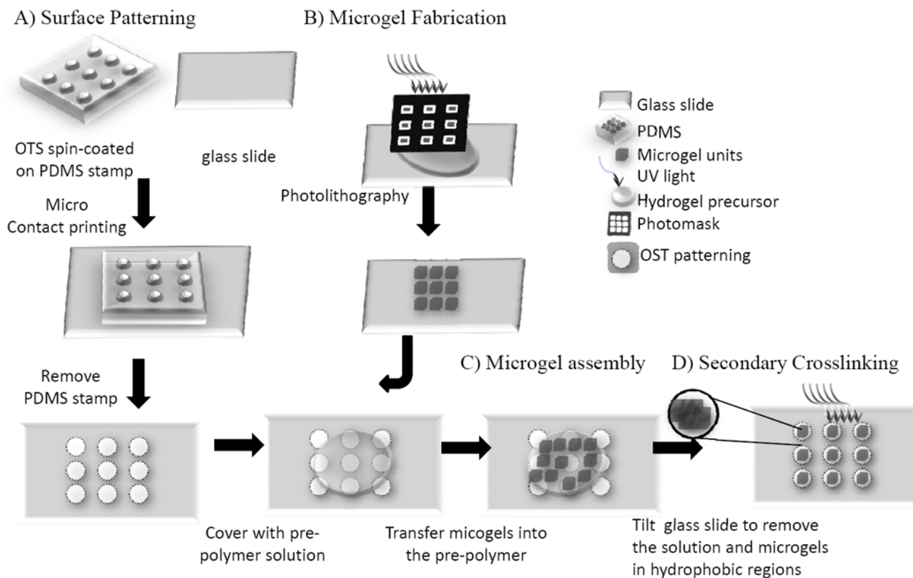
Fig. 1. Schematic diagram of the procedures involved in the surface-directed assembly of microgels (A) generating hydrophobic regions of OTS patterns on a hydrophilic glass by microcontact printing; (B) generating PEG-DA microgel building blocks by photolithography; (C) directed-assembly of the microgels on the hydrophilic patterns; (D) stabilization of the microgel assemblies by secondary crosslinking.
