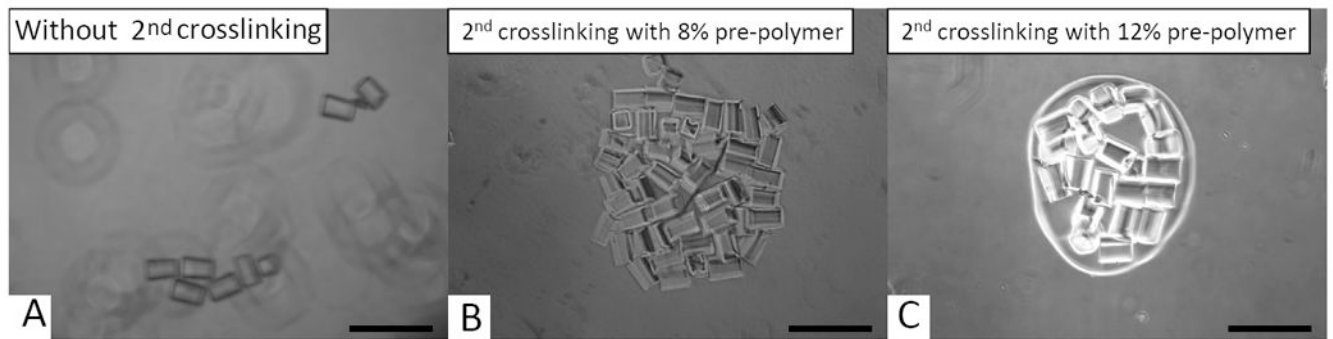
Fig. 4. Secondary crosslinking to encapsulate the assembled microgels in a bulk hydrogel with defined architecture
