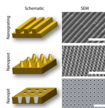
Figure 1. Schematics and SEM Images of Representative Nanotopography Geometries. Three basic nanotopography geometries include nanograting ( 45^\circ tilt, scale bar represents 5\ \mu\text{m} ), nanopost array ( 15^\circ tilt, scale bar represents 5\ \mu\text{m} ) and nanopit array ( 0^\circ tilt, scale bar represents 1\ \mu\text{m} ). Schematics not drawn to scale.
