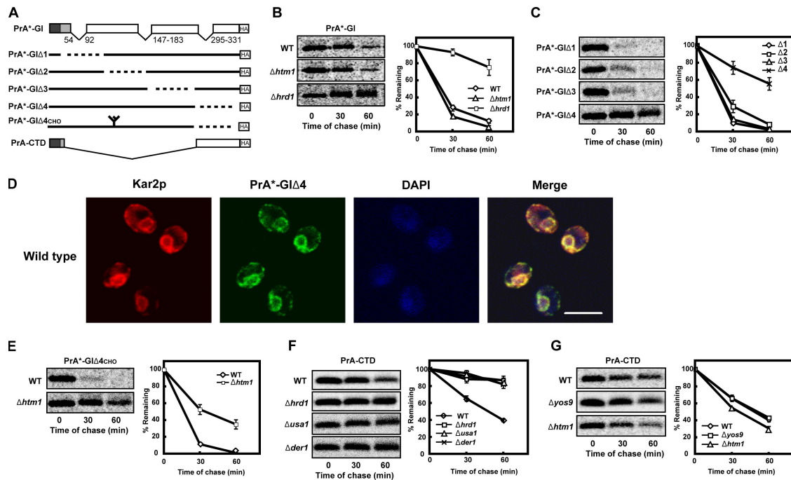
Figure 5. PrA contains a distinct determinant for glycan-independent ERAD. (A) Schematic representation of PrA * -GI variants. N-linked glycans are represented by branched symbols, signal sequences are shaded dark gray, prodomains are colored light gray, and positions of HA epitope tags are indicated. Dashed lines mark deleted regions. (B, C, and E–G) Substrate decay rates were measured and presented as described in Fig. 1 B. Strains and substrates are indicated. (B) PrA * -GI decay rates in wild-type (WT), \Delta htm1 , and \Delta hrd1 cells. (C) Degradation profiles for PrA * -GI \Delta 1, PrA * -GI \Delta 2, PrA * -GI \Delta 3, or PrA * -GI \Delta 4 in wild-type cells. (D) Intracellular localization of PrA * -GI \Delta 4 in wild-type cells was analyzed by confocal microscopy. The substrate was detected using anti-HA antibodies (green), the ER was visualized using anti-Kar2p antisera (red), and nuclei were stained by DAPI. Bar, 5 \mu m. (E) Wild-type and \Delta htm1 cells expressing PrA * -GI \Delta 4 CHO . (F) Wild-type, \Delta hrd1 , \Delta usa1 , and \Delta der1 cells expressing PrA-CTD. (G) Wild-type, \Delta yos9 , and \Delta htm1 cells expressing PrA-CTD. Error bars indicate SEM.
