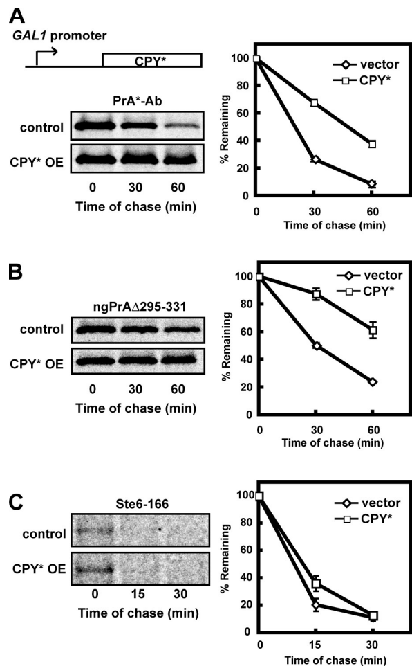
Figure 4. Glycan-independent and glycan-dependent substrates of ERAD-L are competitors for degradation. (A) Wild-type cells carrying GAL1 -regulated CPY * (or nonexpressing control vector) and PrA * -Ab regulated by its native promoter were shifted to galactose media to induce CPY * expression. Turnover of PrA * -Ab was analyzed as described in Fig. 1 B. (B) The experiment was performed as described for A with ngPrAΔ295–331 as the test substrate. (C) The experiment was performed as described for A with Ste6-166p as the test substrate. OE, overexpression. Error bars indicate SEM.
