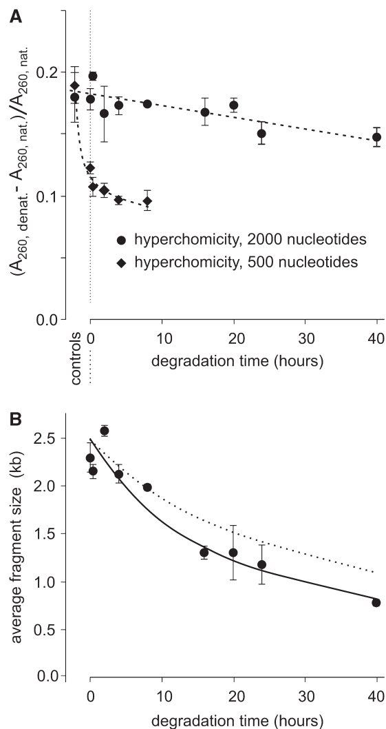
Figure 3. Control for cross-links. (A) Relative hyperchromicity ( A_{260, \text{denat.}} - A_{260, \text{nat.}}/A_{260, \text{nat.}} ) of DNA populations of 2000-nt and 500-nt average sizes of fragments after vacuum drying and heating kinetics at 110°C. Some error bars are smaller than the symbols. The lines serve as visual guides. (B) Average size of the large fragment population measured by denaturing gel electrophoresis. The continuous line was calculated by curve-fitting (giving a corresponding degradation rate of 5.5 \times 10^{-9} \text{ s}^{-1} \text{ nt}^{-1} ). The dotted line represents the decrease in average fragment size calculated from plasmid degradation data (degradation rate: 3.5 \times 10^{-9} \text{ s}^{-1} \text{ nt}^{-1} at this temperature). Some error bars are smaller than the symbols.
