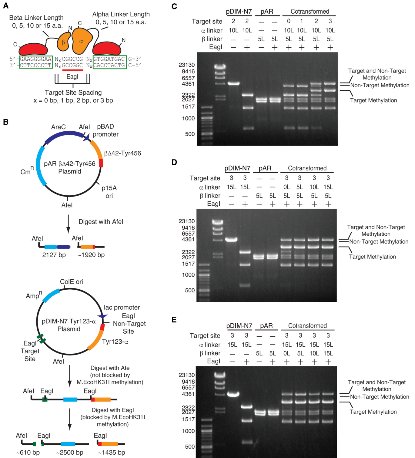
Figure 1. The effect of fusion linker length and spacing at the target site on the methyltransferase activity and specificity of M.EcoHK311 -derived constructs with a 42-residue deletion on the \beta fragment. (A) Schematic of the various constructs tested showing the variability in linker length between zinc finger and methyltransferase fragments and the distance between the zinc finger's binding site and the target site for methylation. (B) The two plasmids encoding the two methyltransferase fragments and the DNA fragments that result from AfeI and EagI digestion if the EagI site is not methylated (methylation blocks EagI but not AfeI digestion). Methylation creates uniquely sized bands depending on if the target or non-target site is protected. Representative results are shown to demonstrate the observed effects of (C) zinc finger-target site distance, (D) linker lengths between the \alpha fragment and Tyr123 and (E) linker lengths between the \beta fragment and Tyr456. Linker lengths are designated by 0, 5, 10 or 15 L and the spacing at the target site designated by the number of base pairs between the target site and zinc finger site. Individual plasmids digested with AfeI are also shown for size comparisons (pDIM-N7 and pAR) with (+) and without (-) EagI digestion. The locations of bands resulting from only target methylation, only non-target methylation and methylation at both sites are indicated. The plasmids were prepared from cells grown in LB media.
