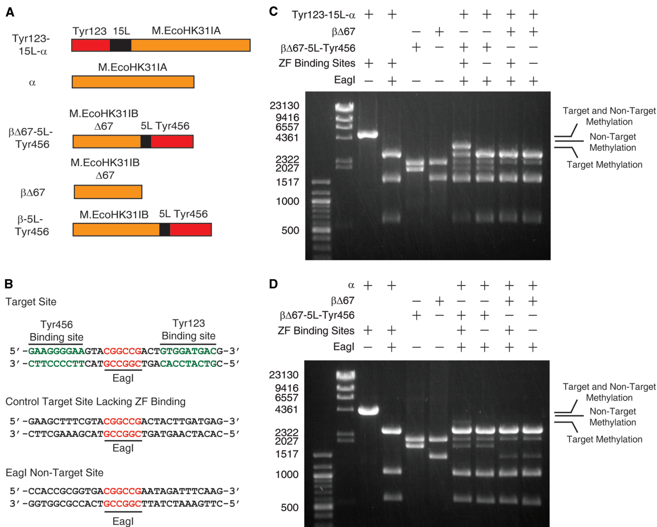
Figure 2. The effects of removing zinc finger proteins or zinc finger binding sites on the methylation activity and specificity of M.EcoHK311-derived constructs with a 67-residue deletion on the β fragment. (A) Schematic of the fusion and control constructs used in these experiments. (B) DNA sequences at the target sites (with and without zinc finger binding sites) and non-target site. All pDIM-N7 plasmids contain a non-target site and either the target site containing zinc finger binding sites (+) or containing a control site for which the zinc fingers lack affinity (-). Gel electrophoresis results for plasmids digested with AfeI and EagI (performed as in Figure 1) are shown for plasmids containing the DNA encoding (C) Tyr123-15L-α and (D) α cotransformed with plasmids encoding βΔ67 or βΔ67-5L-Tyr456. Results for AfeI or AfeI/EagI digestions of unmethylated control plasmids are shown for size comparison. The locations of bands resulting from only target methylation, only non-target methylation and methylation at both sites are indicated. The plasmids were isolated from cells grown in LB media.
