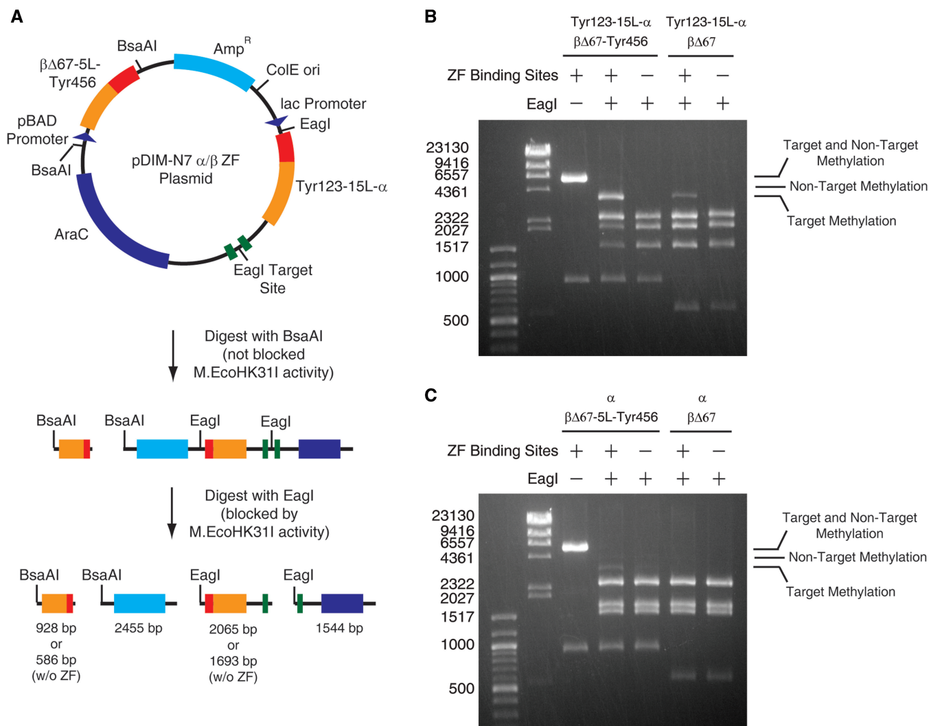
Figure 3. Methylation activity and specificity resulting from a single plasmid encoding Tyr123-15L- \alpha and \beta\Delta 67 -5L-Tyr456 (A). Schematic of the plasmid and its digestion with BsaAI (not-blocked by methylation) and EagI (blocked by methylation). Gel electrophoresis results for plasmids digested with BsaAI and EagI are shown for plasmids contain the DNA encoding (B) Tyr123-15L- \alpha and (C) \alpha Combinations with DNA encoding either \beta\Delta 67 or \beta\Delta 67 -5L-Tyr456 and with and without zinc finger binding sites flanking the target site were tested. The locations of bands resulting from only target methylation, only non-target methylation and methylation at both sites are indicated. Plasmids were isolated from cells grown in LB media supplemented with 0.2% glucose.
