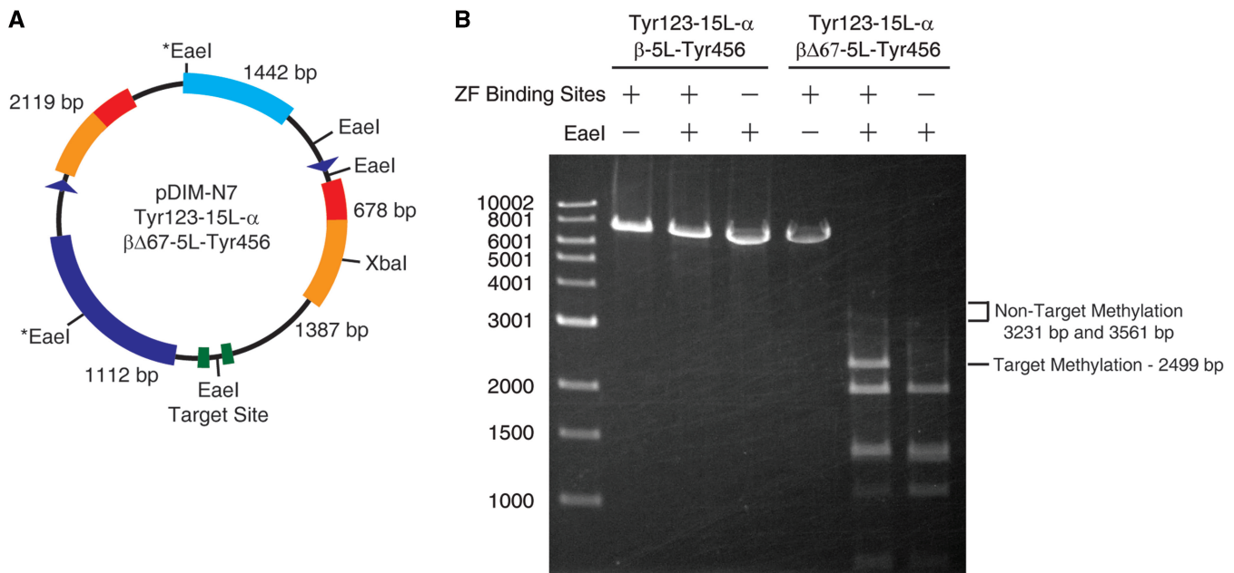
Figure 4. Tyr123-15L- \alpha / \beta\Delta 67-5L-Tyr456 has a high preference for the target site over other M.EcoHK31I methylation sites. (A) The pDIM-N7 plasmid contains five methylation sites for M.EcoHK31I that overlap EaeI restriction enzyme sites (EaeI is blocked by methylation) and one XbaI site used to linearize the plasmid and facilitate analysis. The sizes of the five largest DNA fragments that result from XbaI/EaeI digestion of unmethylated DNA are shown. (B) Agarose gel electrophoresis results of XbaI/EaeI digestions of plasmids expressing Tyr123-15L- \alpha / \beta\Delta 67-5L-Tyr456 or Tyr123-15L- \alpha / \beta -5L-Tyr456 (i.e. control protein with no truncation of the \beta fragment). Methylation at the target site yields a 2499 bp band if the flanking sites are not methylated. Methylation at the two EaeI sites marked with an asterisk would result in bands at either 3231 bp or 3561 bp if their flanking sites are not methylated. These two EaeI sites are non-target sites that were not tested in previous experiments. Plasmids were isolated from cells grown in LB media supplemented with 0.2% glucose.
